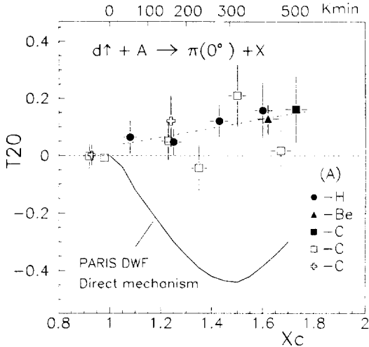
Fig.3. T_{20} vs x_c and k_{min} (MeV/c) for the reaction d + A \rightarrow \pi(0^\circ) + X at the fragmentation of 9 GeV deuterons on the hydrogen, beryllium and carbon targets obtained in this experiment along with the previous data [23] obtained with the carbon target for \pi^- (open squares) and \pi^+ (open cross). The dashed line is a linear fit of the data ( \chi^2/d.o.f.=0.5 ). The solid curve is our calculation based on the Paris DWF [23].
