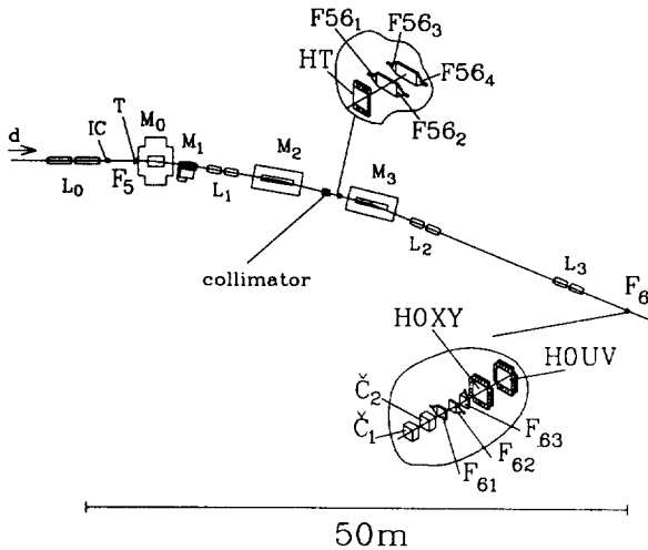
Fig.2. The layout of the setup of the 4V beam line in the Synchrotron experimental hall. M_i ; bending magnets, L_i ; quadrupole magnets, F_i, C_i ; scintillation and Cherenkov counters, HT, HOXY, HOUV ; scintillation hodoscopes, T ; target. IC : ionization chamber.
