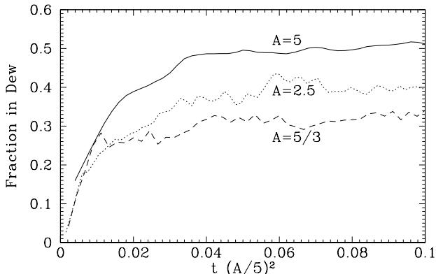
FIG. 2. Condensation process.
