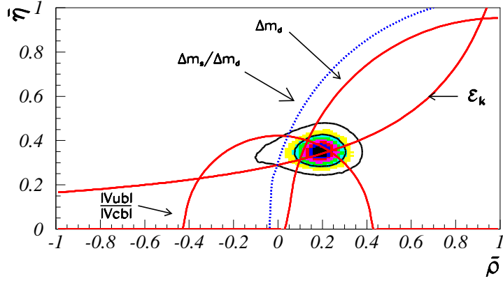
Figure 7: The \bar{\rho} - \bar{\eta} allowed region. The contours at 68% and 95% C.L. are shown. The continuous lines correspond to the constraints obtained from the measurements of \frac{|V_{ub}|}{|V_{cb}|} , \Delta m_d , and \varepsilon_K . The dotted curve corresponds to the 95% C.L. limit obtained from the experimental limit on \Delta m_s .
