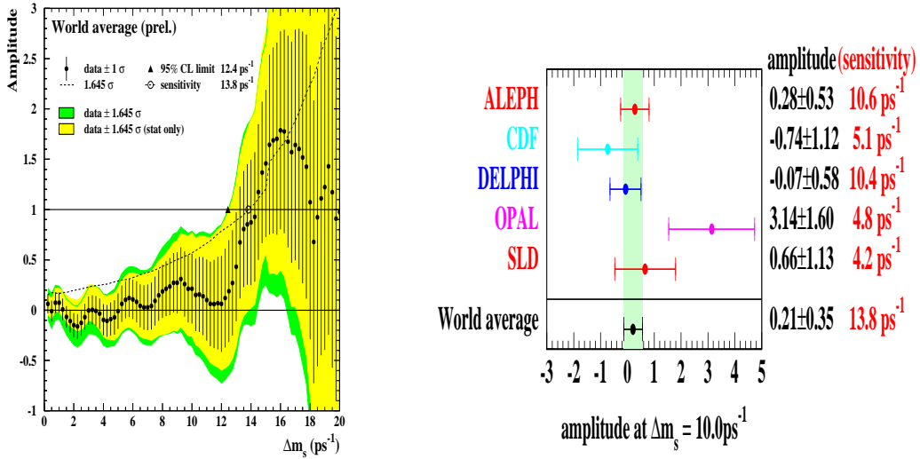
Figure 5: The plot on the left shows the combined \Delta m_s results from LEP/SLD/CDF analyses shown in an amplitude versus \Delta m_s plot. The points with error bars are the data; the lines show the 95% C.L. curves (in dark the systematics have been included). The dotted curve shows the sensitivity. The plot on the right shows the summary of the \Delta m_s results per experiment. The error are given at \Delta m_s = 10 \text{ ps}^{-1} (the sensitivity is also given). The way in which the combined value is obtained is described in [1].
