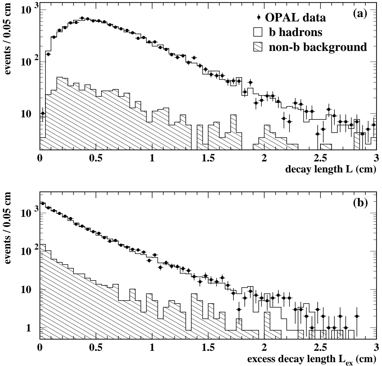
Figure 3: Distributions of (a) decay length L and (b) excess decay length L_{\text{ex}} in data (points with error bars) and Monte Carlo (histogram), for all selected secondary vertices. The expected contributions of b hadrons and non- b background are indicated.
