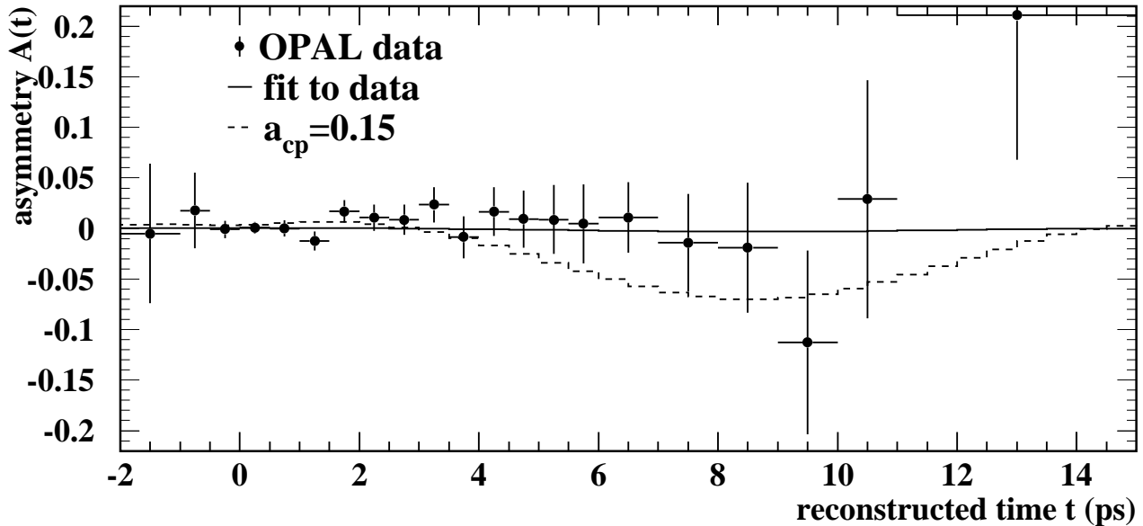
Figure 8: Asymmetry of tagged b and \bar{b} hadrons as a function of reconstructed time t in data (points), and fit (solid line). The expected asymmetry for a_{\text{cp}} = 0.15 is shown by the dotted line.
