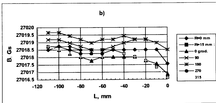
Fig. 2. Results of measurements of the magnetic field in the working volume of the target ( I_{\text{main}} = 74.42 A; I_{\text{cor.1}} = 2.60 A; I_{\text{cor.2}} = 4.64 A).
