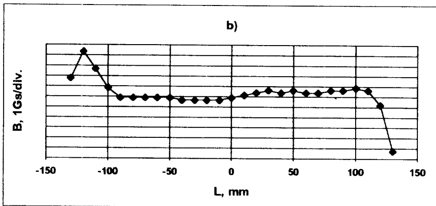
Fig. 3. Results of measurements of the magnetic field in the working volume of the target using an additional "warm" correction
