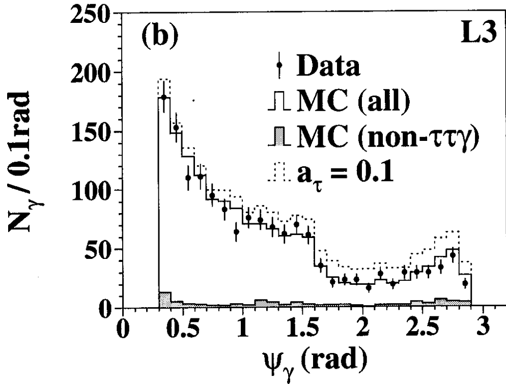
Figure 2: The number N_\gamma of photon candidates in the e^+e^- \rightarrow \tau^+\tau^-\gamma sample as a function of (a) photon energy E_\gamma and (b) the isolation angle \psi_\gamma defined in the text. The points with error bars denote the data and the solid histograms denote the Monte Carlo predictions, assuming the SM values of a_\tau and d_\tau . For illustration, the dashed histograms show how the distributions would appear for a_\tau = 0.1 . Both the increase in the total cross section and the relatively greater importance of photons with large E_\gamma and \psi_\gamma are evident.
