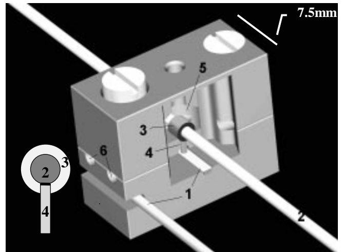
Figure 4: Tip heater drawing: 1 heater current lead, 2 sample, 3 thermo-retracting sleeve (optional), 4 heater tip, 5 helium reservoir (connected to the bath through a channel), 6 helium channels. The heater tip is squeezed between sample on top and the heater current lead from below. The heater current lead acts as a spring.
