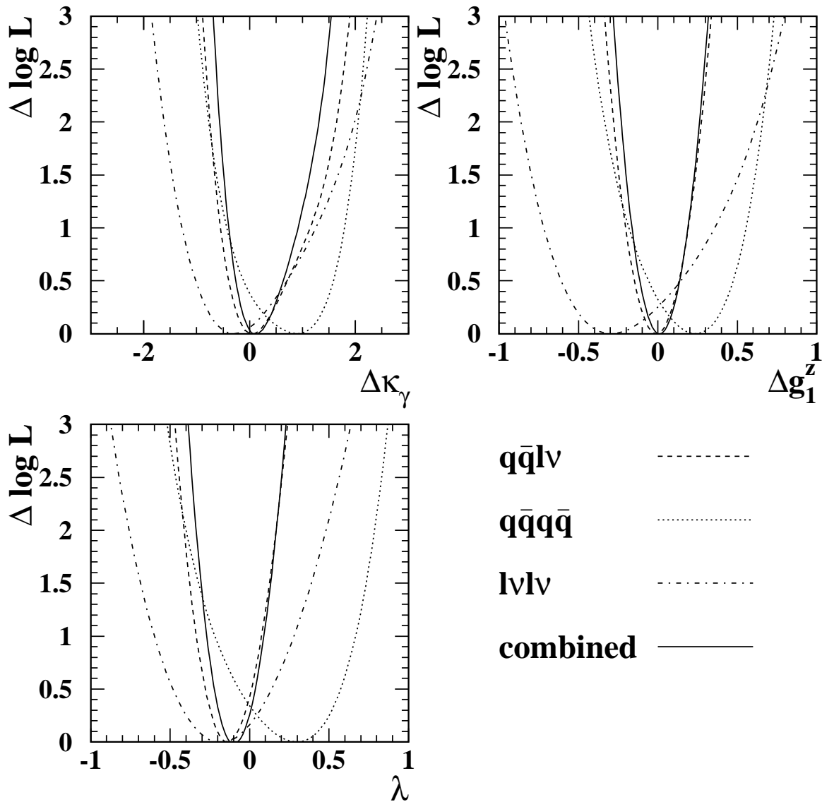
Figure 11: Negative log-likelihood curves obtained in the different event selections: q\bar{q}\bar{\ell}\nu_\ell (dashed lines), q\bar{q}q\bar{q} (dotted lines) and \bar{\ell}\nu_\ell\ell'\bar{\nu}_\ell (dash-dotted lines). Each curve is obtained by combining the results from the angular distributions and the cross-section and setting the other two TGC parameters to zero. Systematic errors are included. The solid line is obtained by combining the three event selections.
