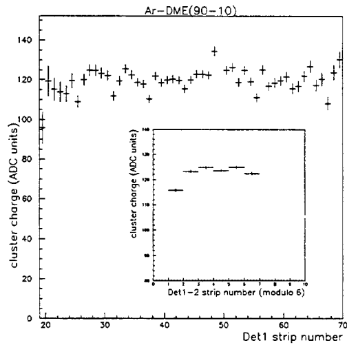
Figure 8: Micromegas response on the strip which gives the highest signal in a cluster. Inset: the mean response on modulo 6 strips. Strips with a spacer are marked with a dot.
