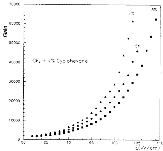
Figure 16: Gain as a function of the amplification electric field with a gas mixture of different cyclohexane concentrations in CF 4 .
