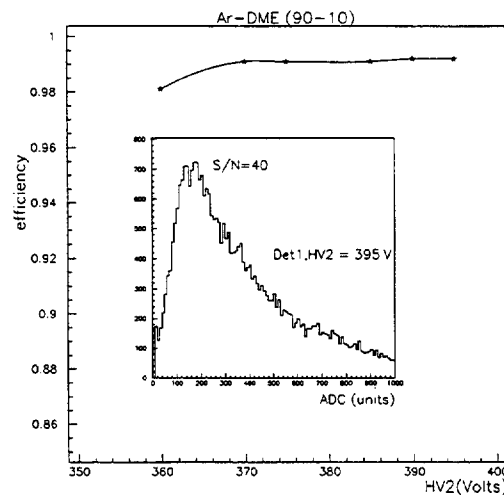
Figure 9: Efficiency plateau. Inset: the response distribution at 395 V.
