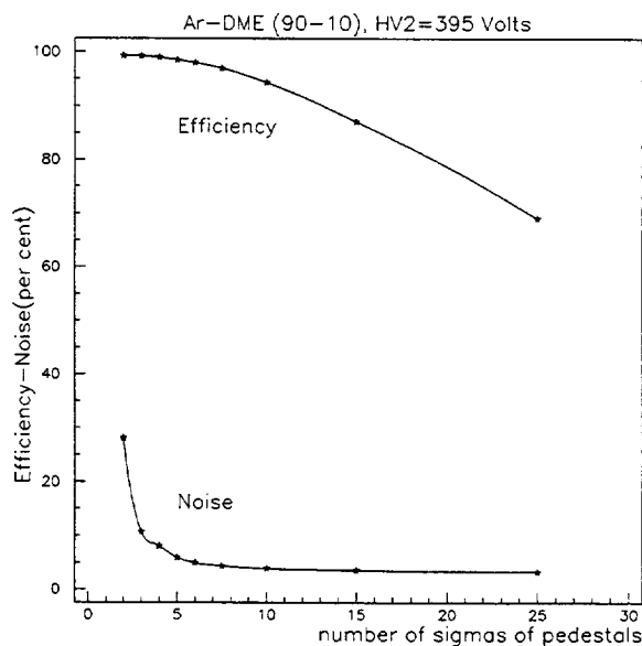
Figure 7: Efficiency and fraction of noisy strips as a function of the strip noise threshold.
