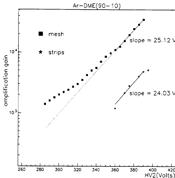
Figure 6: Gain measured on mesh (in laboratory) and on strips (in beam) as a function of the mesh potential.
