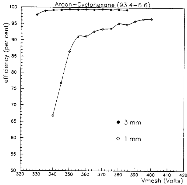
Figure 15: Efficiency plateau for 3-mm and 1-mm conversion gaps.
