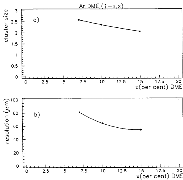
Figure 12: Variation as a function of DME concentration of a) the cluster size and b) the spatial resolution.
