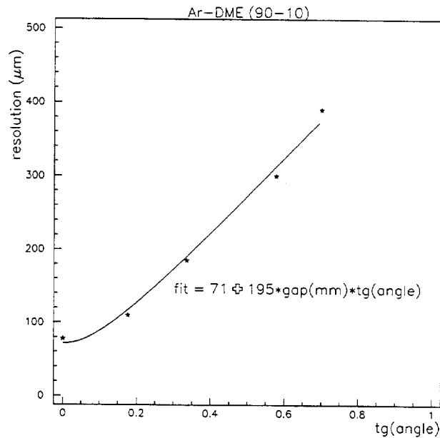
Figure 13: Spatial resolution as a function of the tangent of the track angle. The fit is the square root of the quadratic sum of two terms.
