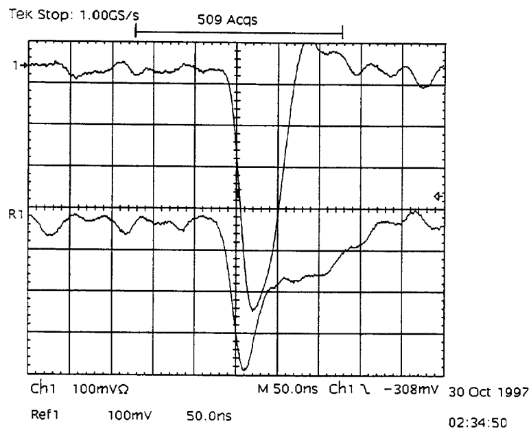
Figure 4: Signal given by the MQS104A chip, for 50- \mu\text{m} (top) and 100- \mu\text{m} (bottom) amplification gaps.
