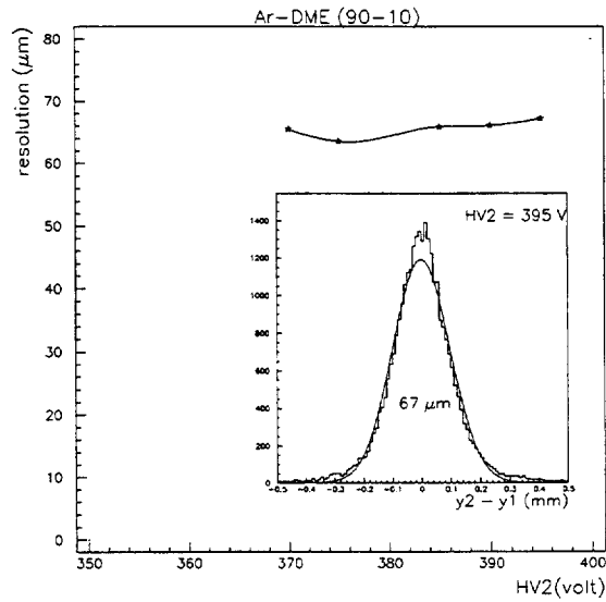
Figure 11: Spatial resolution as a function of the mesh potential. Inset: the difference between the two centroids in the doublet at 395 V.
