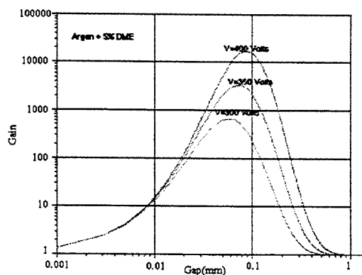
Figure 2: Expected gain as a function of the amplification gap at various potentials.
