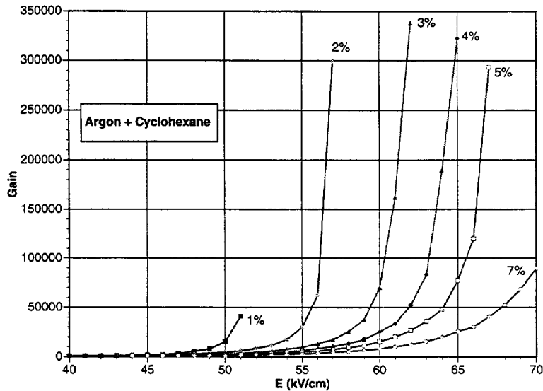
Figure 14: Gain as a function of the amplification electric field for different cyclohexane concentrations in argon.
