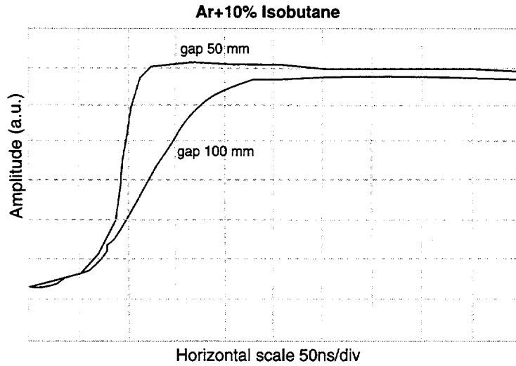
Figure 3: Signal given by a charge preamplifier, for 50 and 100 \mu\text{m} amplification gaps.
