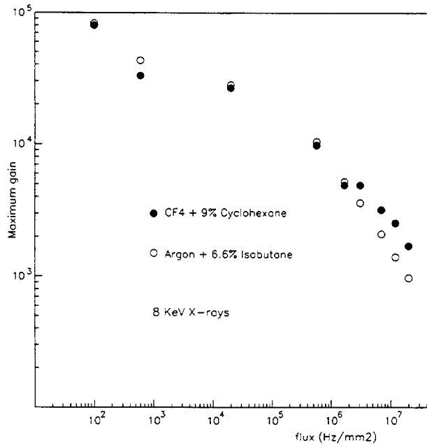
Figure 17: Maximum gain as a function of 8 keV X-ray flux.
