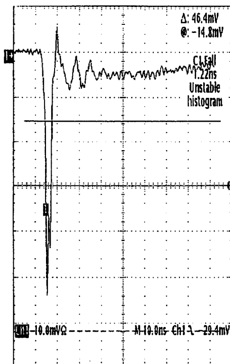
Figure 5: Signal given by a current preamplifier.
