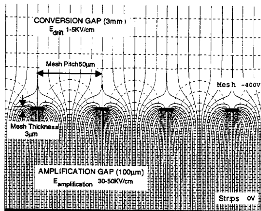
Figure 1: Micromegas electric-field map.
