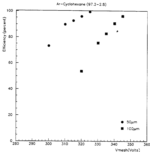
Figure 18: Efficiency as a function of the mesh potential measured with the MQS104A chip, for 100- \mu\text{m} and 50- \mu\text{m} amplification gaps.
