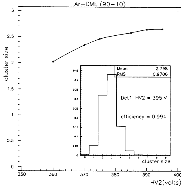
Figure 10: Cluster size as a function of the mesh potential. Inset: the strip multiplicity distribution at 395 V.
