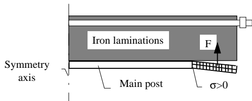
Figure 4: The bending effect in the coil end
