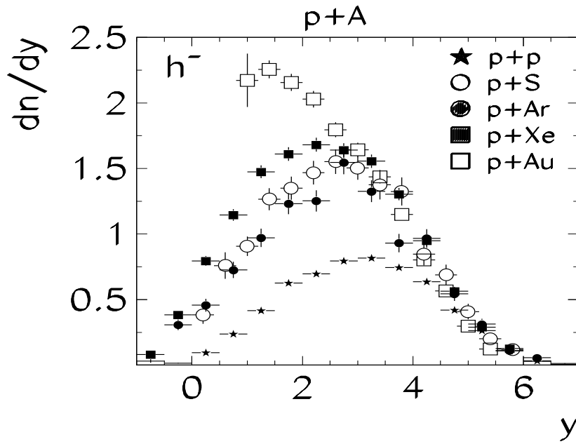
Figure 21. Rapidity distributions of negatively charged hadrons produced in minimum bias p+p, p+S, p+Ar, p+Xe and p+Au collisions [36]. Note that the rapidity distribution for p+S collisions is higher than for p+Ar interactions due to different trigger conditions and event selections.
