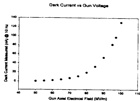
Figure 10: Measured dark current at the down stream against the surface field. It shows the exponential dependence and the maximum dark current observed was 13 nC at 100 MV/m.
