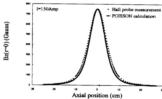
Figure 6: Longitudinal solenoid field profile on axis.
