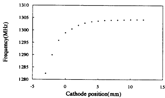
Figure 4: Measured resonant frequency to the cathode plug position.
