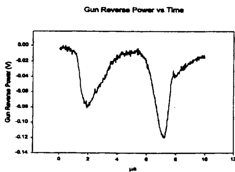
Figure 9: Reflected rf power from the gun. It shows that
