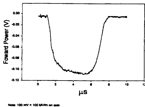
Figure 8: Measured forward rf power to the gun. The voltage measures 2 MW rf peak power.
