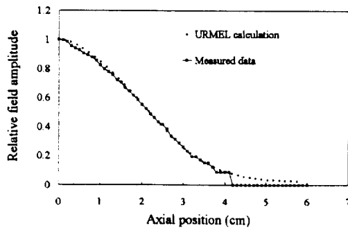
Figure 5: Longitudinal E-field profile on axis.
