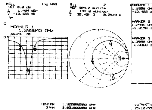
Figure 2: Measured reflection coefficient of gun cavity.
