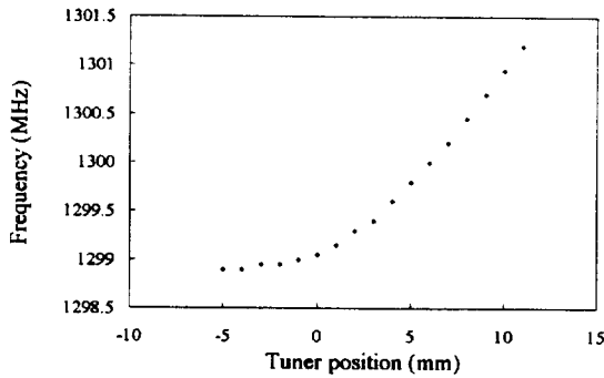
Figure 3: Measured resonant frequency to the tuner position.
