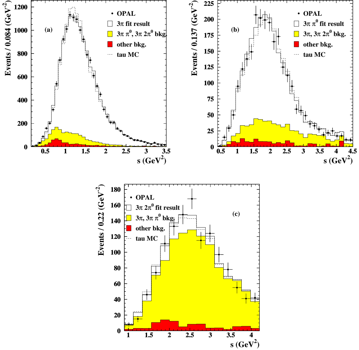
Figure 3: The measured s_{meas} spectra for 3-prong decays. Plot (a) is the 3\pi channel, (b) and (c) are the 3\pi\pi^0 and 3\pi2\pi^0 modes, respectively. The points denote OPAL data (statistical errors only). The open histograms show the fitted spectra after the regularized unfolding, refolded into detector space. The background contributions from simultaneously unfolded channels (correlated background) are shown as light grey areas while the background from other sources (uncorrelated background) is represented in dark grey.
