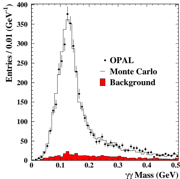
Figure 1: The \gamma\gamma -mass in the \pi\pi^0 channel for decays with two reconstructed photons with a minimal energy of 0.5\text{ GeV} . OPAL data is shown as data points; the total Monte Carlo prediction is given by the open histogram and the shaded histogram denotes the \tau and non- \tau background.
