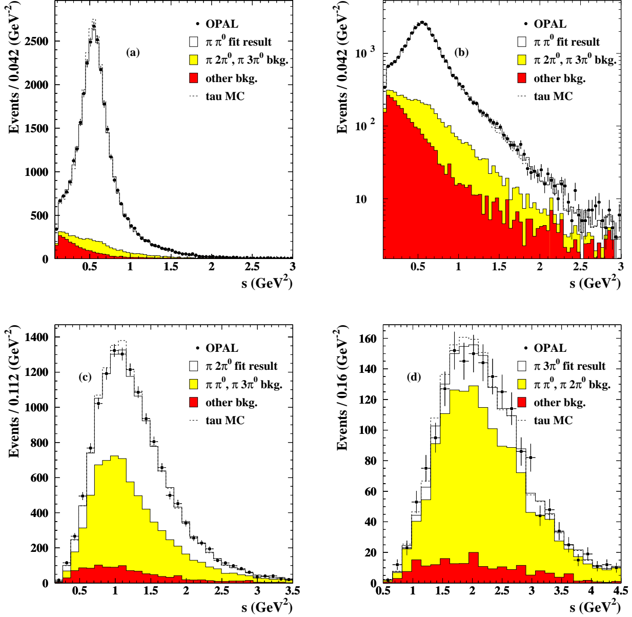
Figure 2: The measured s_{meas} spectra for 1-prong decays. Plots (a) and (b) are the \pi\pi^0 channel, (c) and (d) are the \pi 2\pi^0 and \pi 3\pi^0 modes, respectively. The points denote OPAL data (statistical errors only). The open histograms show the fitted spectra after the regularized unfolding, refolded into detector space. The background contributions from simultaneously unfolded channels (correlated background) are shown as light grey areas while the background from other sources (uncorrelated background) is represented in dark grey.
