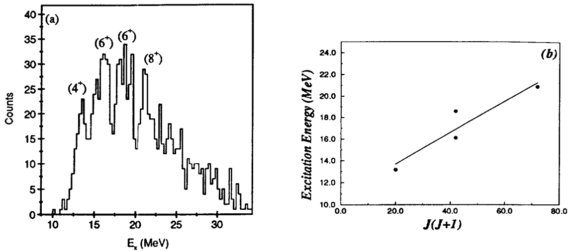
FIGURE 1. (a) ^{12}\text{Be} excitation energy spectrum for ^6\text{He}+^6\text{He} coincidences, (b) the energy-spin systematics of the breakup states.
