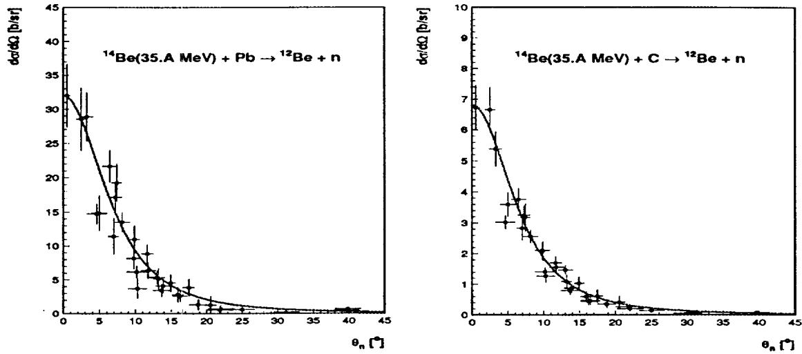
FIGURE 2. Single neutron angular distributions for the breakup of ^{14}\text{Be} ( E_n=10 to 100 MeV).
