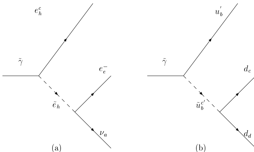
FIG. 1. Diagram for gaugino decay into (a) three leptons ( \Delta L = 1 ), which occurs for the P'_1 P'_2 P'_3 direction; (There are similar diagrams for decay into td_d^c e_a^- or bd_d^c \nu_a .) (b) three quarks ( \Delta B = 1 ), which occurs for the P_2 P_3|_F direction. u'_b , d_c and d_d are SU(2) singlets (i.e., the conjugates of u_b^c , d_c^c and d_d^c ).
