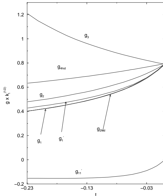
FIG. 2. Running of the gauge couplings \times\sqrt{k} for the P'_1P'_2P'_3 flat direction, with t = 1/16\pi^2\ln(\mu/M_{String}) , with M_{string} = 5 \times 10^{17} GeV, g_{1M_{string}} = 0.80 . The couplings include the factor \sqrt{k} , where k corresponds to the Kač-Moody level (see the caption of Table V for the values of k ).
