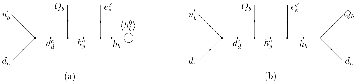
FIG. 3. Proton decay diagrams for (a) \langle h_b^0 \rangle \neq 0 , (b) \langle h_b^0 \rangle = 0 . u'_b, d_c are the conjugates of u_b^c, d_c^c .
