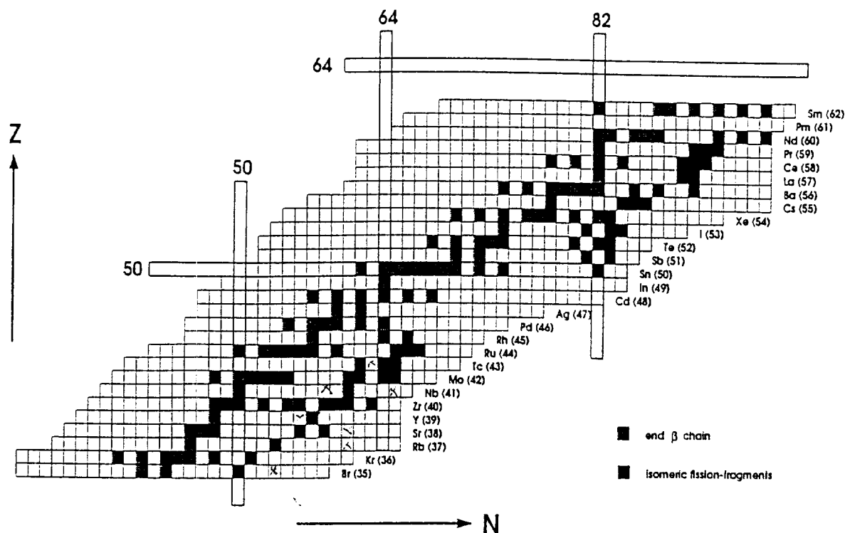
Fig. 3. In this Z-N chart of nuclei \beta stable nuclei are colored in grey. In black are shown nuclei where isomeric states have been identified in the spontaneous fission of ^{252}\text{Cf} . (this work)
