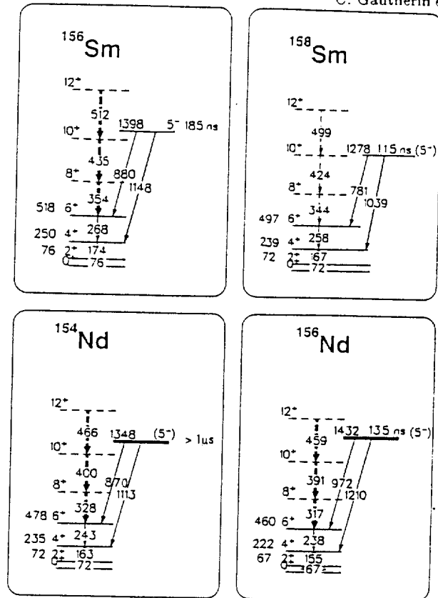
Fig. 6. Partial level schemes of 156,158 Sm and 154,156 Nd (prompt transitions are marked with dashed lines).
