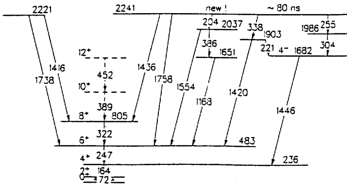
Fig. 5. Partial level scheme of 152 Nd (prompt transitions are marked with dashed lines).
