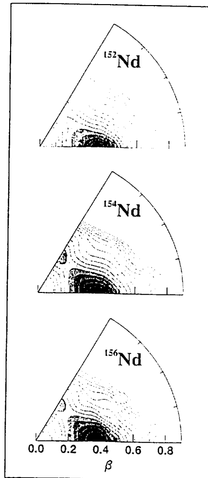
Fig. 7. PES V(\beta, \gamma) for ^{152,154,156}\text{Nd} isotopes.
