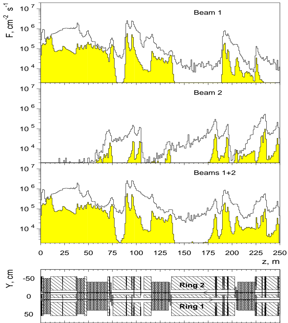
Figure 2: Hadron flux density around the beam lines. Clear histograms - the case without shielding, grey histograms - the case with shielding. The z-range covers a half of the straight section. Beam enters at z=0 , where the primary collimators are located. F(z) in z=[250,500] for beam 2 is similar to F(z) for beam 1 left-right reflected.
