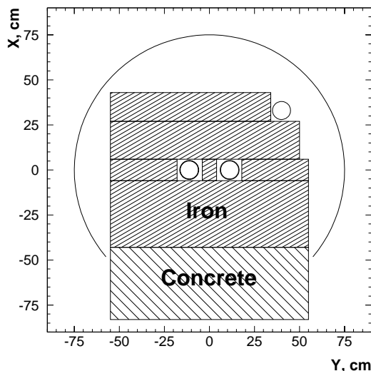
Figure 1: The shielding cross-section. The small central circles are the beam pipes in drift sections. The upper right circle is a survey device. The large circle is a scoring surface.
