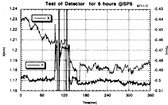
Figure 6: Results of the beam test at SPring 8
