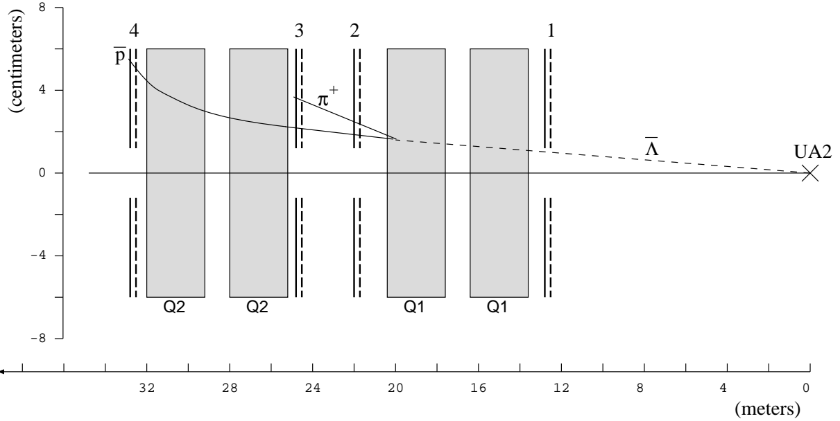
Figure 1: General layout of the two UA8 spectrometers installed in the outgoing \bar{p} -arm with a typical \bar{\Lambda}^{\circ} event, shown decaying in the vertical plane, in the UP spectrometer (drawn with different vertical and horizontal scales). The horizontal axis is the longitudinal z -axis. The vertical axis is the y -coordinate. Q1 and Q2 are each pairs of quadrupole magnets, The four chamber packs (solid vertical lines) each consist of six wire planes as described in Ref. [10], are positioned before and after each magnet at the longitudinal positions shown. Scintillation counters (dashed vertical lines) are installed next to each chamber pack.
