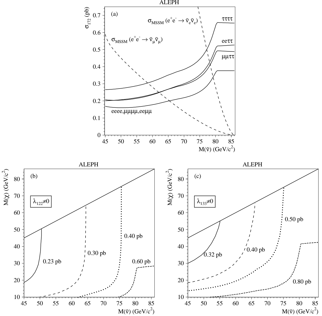
Figure 9: The 95% C.L. sneutrino exclusion cross sections scaled to \sqrt{s} = 172 \text{ GeV} . For the purpose of these plots a \beta^3/s cross section dependence, valid for scalar pair-production in the s-channel, was assumed. Fig. a) shows \sigma_{\text{excluded}}^{172} for the direct decays of sneutrinos. Superimposed are the MSSM cross sections at \tan\beta = 2 for electron-sneutrino production ( M_2 = 100 \text{ GeV}/c^2, \mu = -200 \text{ GeV}/c^2 ) and muon-sneutrino production. Fig. b) and c) show contours of \sigma_{\text{excluded}}^{172} for the indirect decays in the (M_\chi, M_{\tilde{\nu}}) plane for the best-case exclusion ( \lambda_{122} ) and the worst-case exclusion ( \lambda_{133} ).
