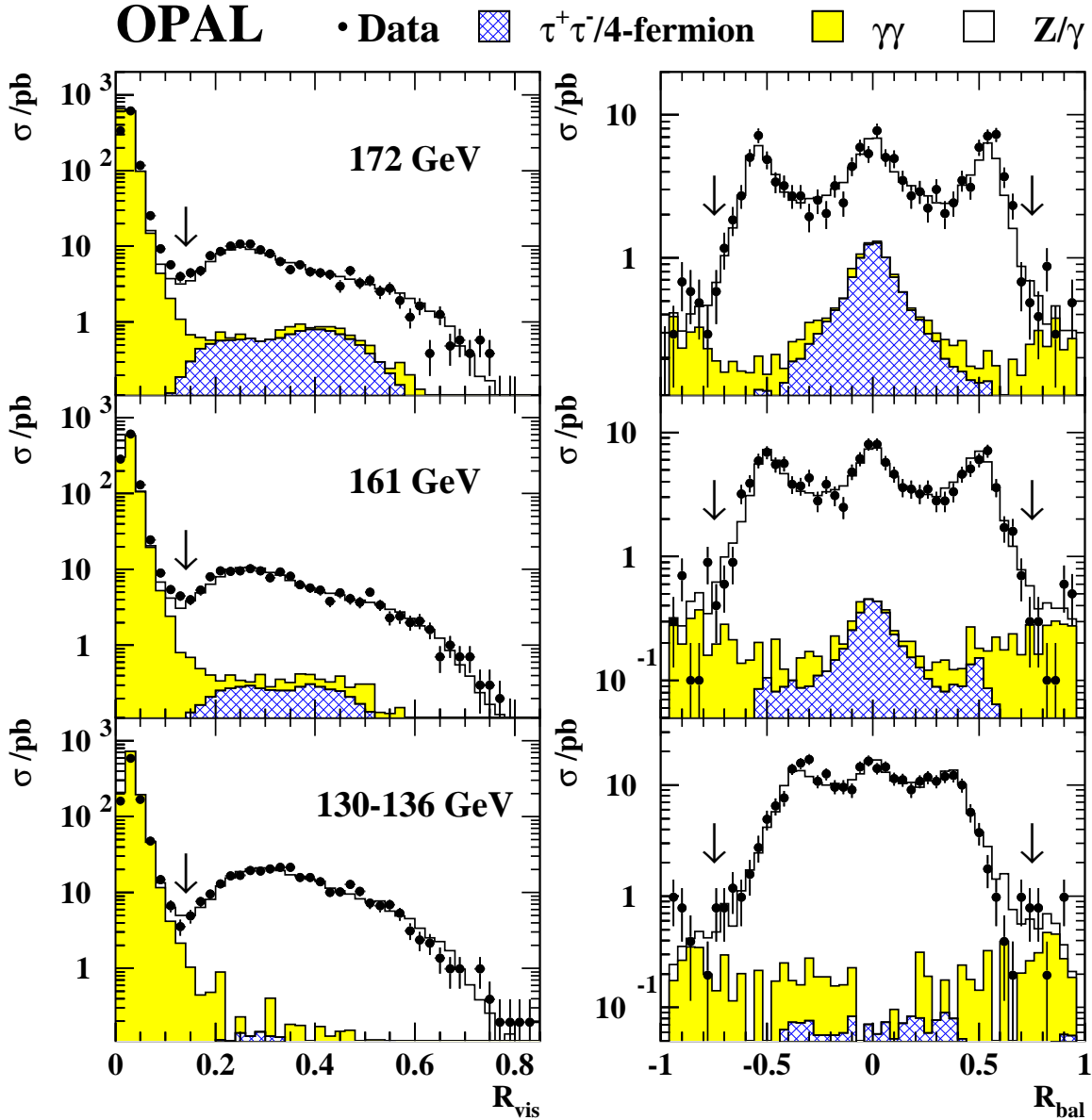
Figure 2: The distributions of R_{\text{vis}} , the ratio of the total energy deposited in the electromagnetic calorimeter to the centre-of-mass energy, and R_{\text{bal}} , the energy imbalance along the beam direction, for hadronic events at each energy. Distributions are shown after all event selection cuts except the cut on that quantity. The positions of the cuts are indicated by the arrows. Points show the data and histograms the Monte Carlo expectations, normalized to the integrated luminosity of the data, with light shading indicating background from two-photon events and cross-hatching indicating other backgrounds, mainly four-fermion (including WW) and \tau^+\tau^- events.
