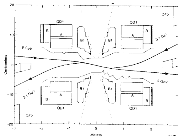
Figure 6B. PEP-II collision point layout
