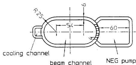
Figure 3A. KEKB HER Cu vacuum chamber
