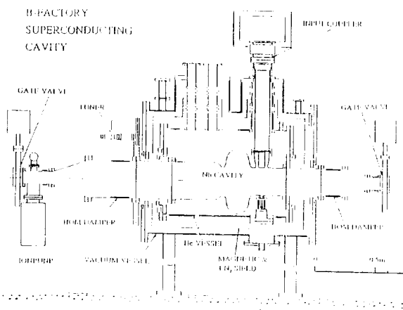
Figure 2B. KEKB superconducting cavity
