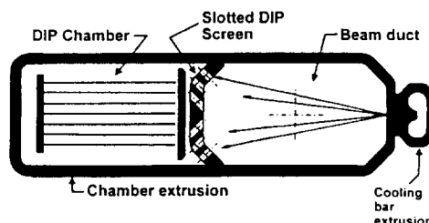
Figure 3B. PEP-II HER Cu dipole chamber
