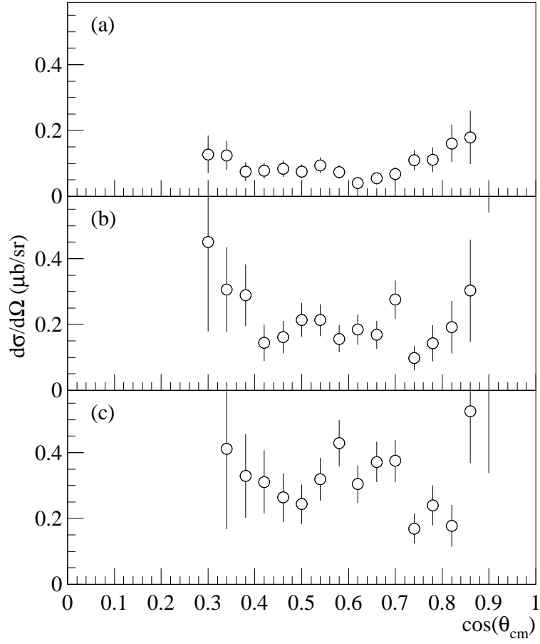
FIG. 6. Differential cross section results for three energy groupings of the reaction \bar{p}p \rightarrow K_s K_s . The 1.2, 1.3, 1.4 and 1.5 GeV/c data are shown in (a), the fine scan 1.39-1.48 GeV/c data are shown in (b) and the 1.6, 1.7, 1.8 and 1.9 GeV/c data are shown in (c).
