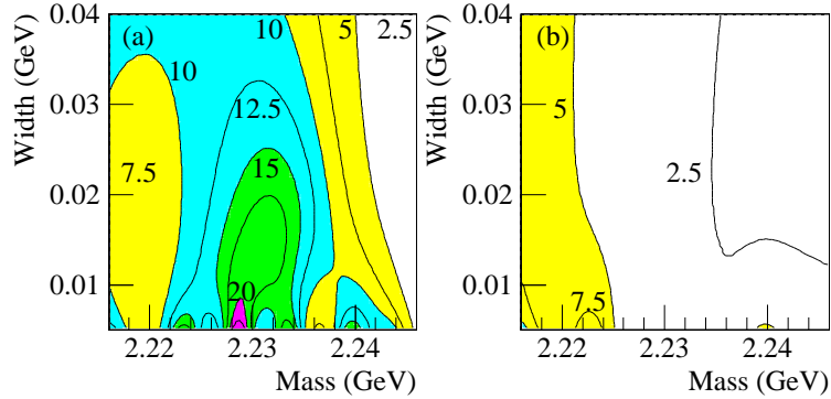
FIG. 7. Contours of the upper limit on the double branching ratio \text{BR}(\xi \rightarrow \bar{p}p) \times \text{BR}(\xi \rightarrow K_s K_s) as a function of resonance mass and width for a J = 2 resonance. The contours represent steps of 2.5 \times 10^{-5} and the shading changes in steps of 5 \times 10^{-5} . In (a) only the data from this work are considered. In (b) our data are combined with the data from PS185 [8] and the same procedure is repeated.
