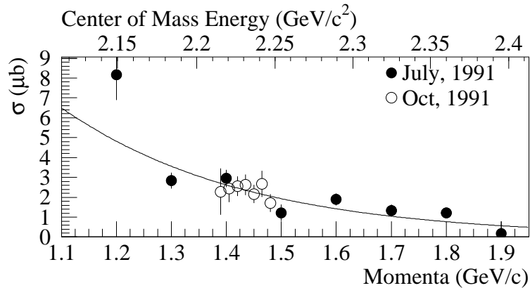
FIG. 5. Total cross section for the reaction \bar{p}p \rightarrow K_s K_s . The solid curve is a fit following the form Ap^* \times e^{-Bp^*} , excluding the 1.2 GeV/c point. The fine-scan data have been adjusted to match the scale of the coarse-scan by means of a multiplicative factor.
