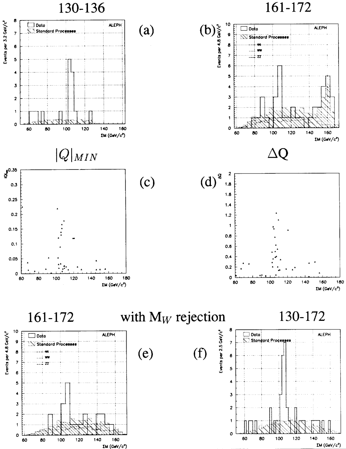
Figure 1: The ALEPH four-jet story
