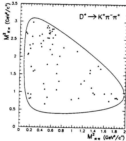
FIG. 4. Dalitz plot ( M^2(K^+\pi^-) vs. M^2(\pi^+\pi^-) ) of events found within 30 MeV/ c^2 of the D^+ mass. This sample corresponds to the events in the shaded region of the dotted histogram shown in Figure 2.
