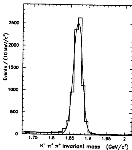
FIG. 3. Mass spectrum of candidate D^+ \rightarrow K^- \pi^+ \pi^+ events with final optimized selection criteria. The curve is a fit to a Gaussian signal and a linear background. The DCS D^+ \rightarrow K^+ \pi^- \pi^+ signal was normalized to this signal.
