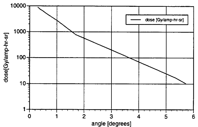
Figure 2 Dose at various positions inside the insertion device
