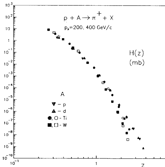
Figure 6. Scaling functions H_A(z) for \pi^+ -meson production in the pA interactions at p_p = 200 and 400 \text{ GeV}/c . Experimental data on inclusive differential cross sections are taken from Ref. [22].
