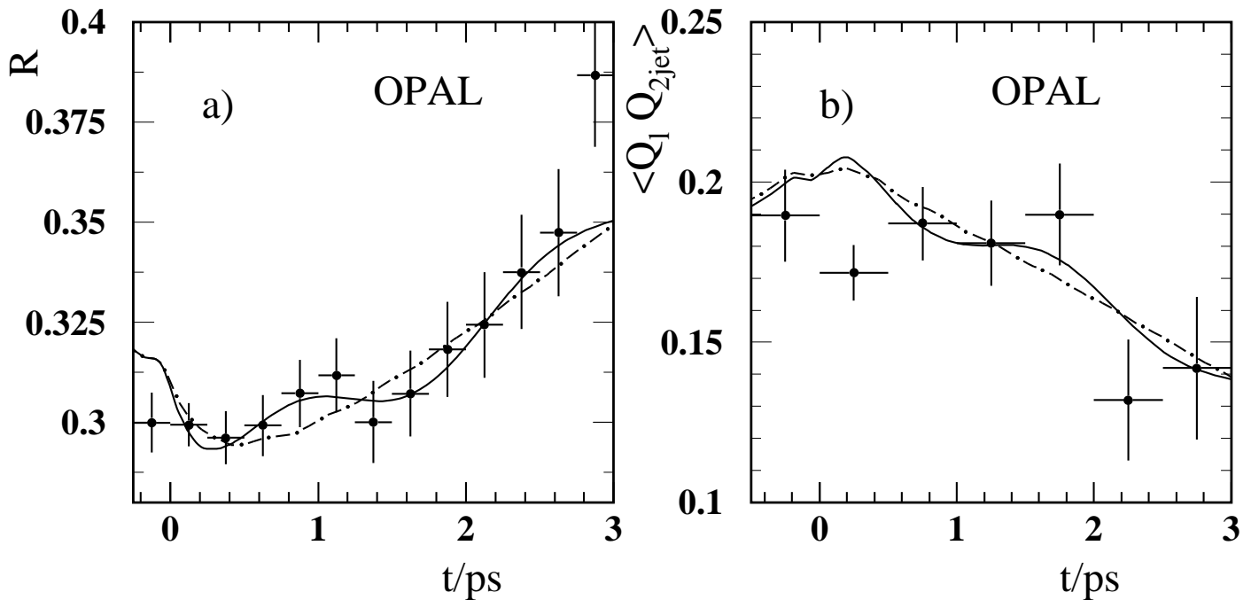
Figure 10: a) The ratio R versus t for data with |Q_{2jet}| > 2 , restricted to the time window -0.25 \text{ ps} < t < 3 \text{ ps} . b) The value of \langle Q_l Q_{2jet} \rangle versus t for data with |Q_{2jet}| < 2 , for the time window -0.5 \text{ ps} < t < 3 \text{ ps} . The solid line shows the result of the fit when \Delta m_s = 3.6 \text{ ps}^{-1} , and the dashed-dotted line corresponds to \Delta m_s = 15 \text{ ps}^{-1} .
