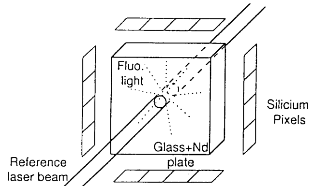
Figure 1: Principle of the SATRAPs. The glue is not shown.
