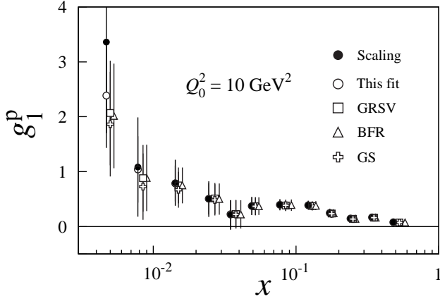
FIG. 18. The structure function g_1^p evolved to Q_0^2 = 10 \text{ GeV}^2 using the scaling assumption that g_1/F_1 is independent of Q^2 , and using NLO evolution according to our analysis and those of BFR [31], GRSV [100] and GS [101].
