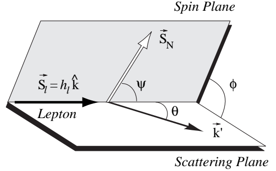
FIG. 1. Lepton and nucleon kinematic variables in polarized lepton scattering on a fixed polarized nucleon target.
