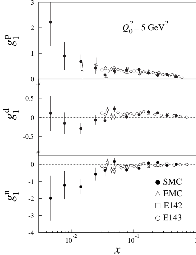
FIG. 19. Measurements of g_1^p , g_1^d and g_1^n evolved to Q_0^2 = 5 \text{ GeV}^2 . The SMC and E143 g_1^n data are obtained from g_1^p and g_1^d .
