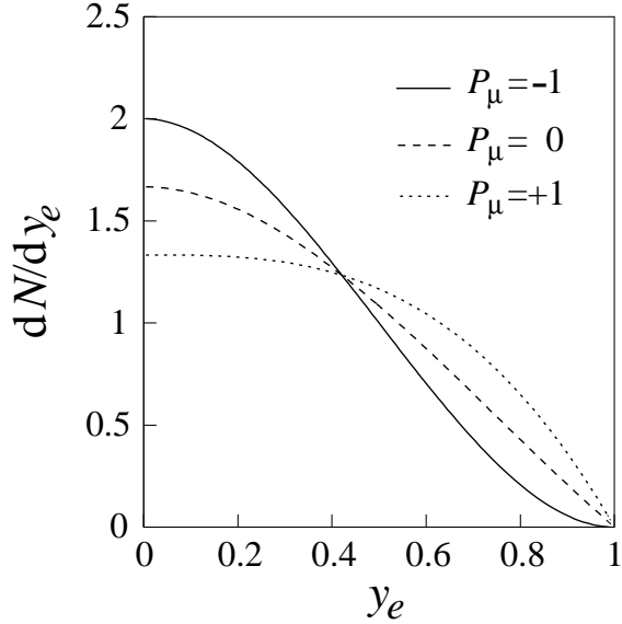
FIG. 5. The Michel spectrum predictions for P_\mu = -1, 0, and +1 are shown by the solid, dashed and dotted lines, respectively.
