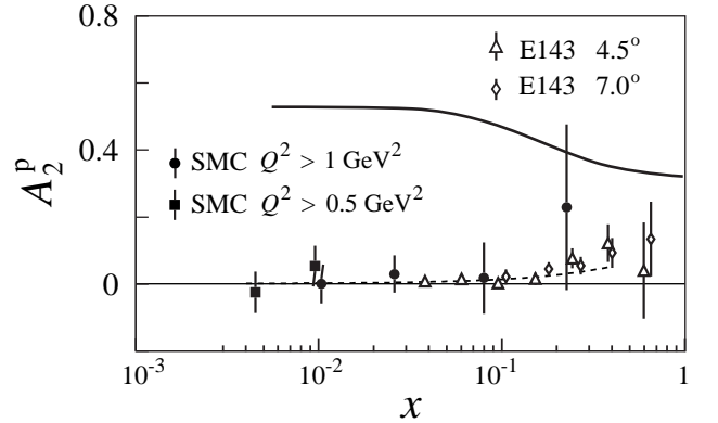
FIG. 15. Results for the asymmetry A_2^P(x) extrapolated to Q_0^2 = 5 \text{ GeV}^2 assuming \sqrt{Q^2} A_2^P scales [10]. The solid and dashed curves show the limit |A_2| < \sqrt{R} and the prediction corresponding to \bar{g}_2 = 0 , respectively. Also shown are data from the E143 experiment [41] extrapolated to the same Q_0^2 assuming that \sqrt{Q^2} A_2 scales. The errors are statistical only.
