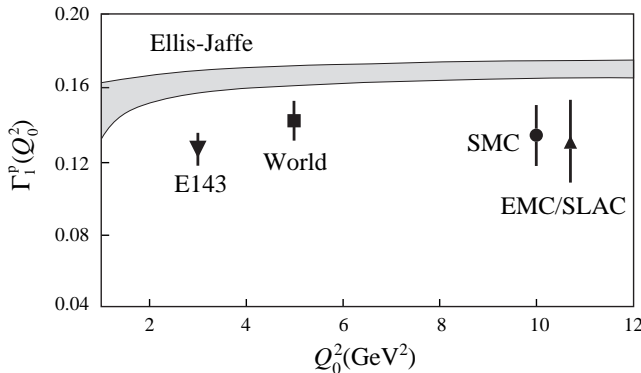
FIG. 20. Comparison of the experimental results for \Gamma_1^p to the prediction of the Ellis–Jaffe sum rule.
