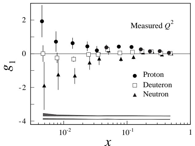
FIG. 16. The structure functions g_1^p and g_1^d at the measured Q^2 and the corresponding g_1^p . The upper and lower shaded areas represent the systematic error for g_1^p and g_1^d , respectively.
