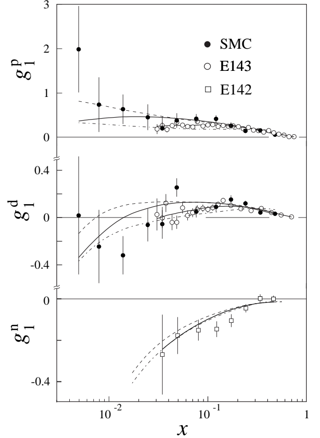
FIG. 17. The structure functions g_1^p , g_1^d , and g_1^n at the measured Q^2 for the SMC [13], E143 [6, 7] and E142 [107] data. The solid curves correspond to our NLO fits at the Q^2 of the data points, the dashed curve at Q_0^2 = 10 \text{ GeV}^2 , and the dot-dashed curve at Q_0^2 = 1 \text{ GeV}^2 .
