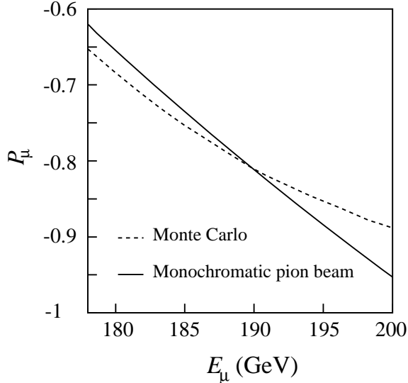
FIG. 3. Muon polarization P_\mu as a function of muon beam energy E_\mu [60] for a monochromatic pion beam of 205 GeV (solid line)(Eq. (3.1)), and mean P_\mu vs. E_\mu as calculated by beam transport simulations [60] (dashed line).
