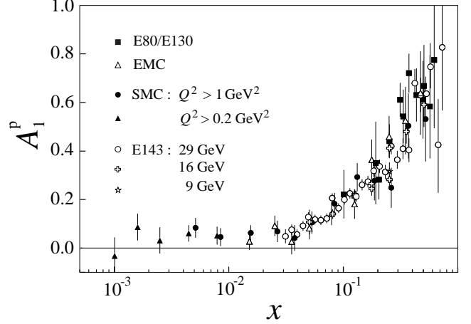
FIG. 14. The virtual photon-proton asymmetry A_1^P as a function of x from this experiment, compared with data from the EMC and the SLAC E80, E130, and E143 experiments. For E143, the structure function ratio g_1^P/F_1^P is shown instead of A_1^P . The errors are statistical only.
