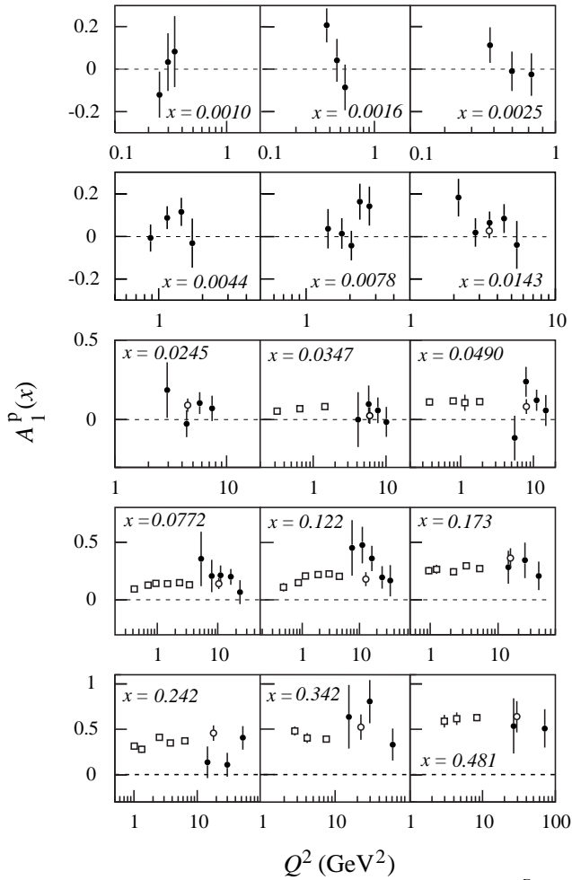
FIG. 13. The virtual photon-proton asymmetry A_1^P as a function of Q^2 , for constant values of x . The closed circles are data from this experiment. The data of the EMC and E143 experiments are also shown as open circles and squares, respectively.
