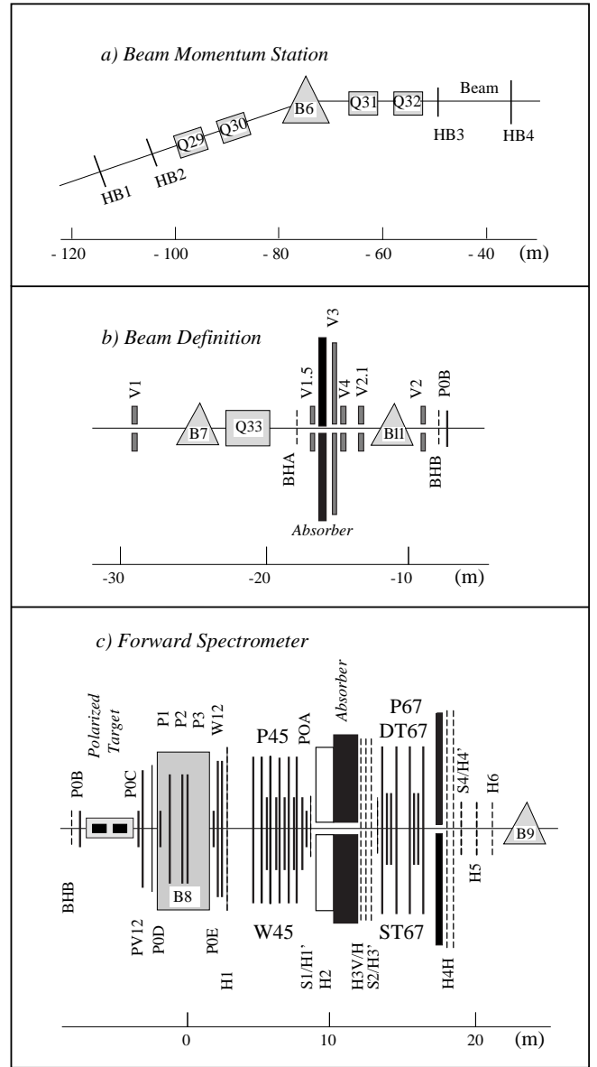
FIG. 2. Schematic layout of the muon beam and forward spectrometer. The individual detectors are discussed in the text (see Table III). In (b), B11 is a compensating dipole that is used only when taking data with transverse target polarization. In (c), B8 is the forward spectrometer magnet and referred to as the FSM in the text. A right-handed coordinate system is used with its origin at the center of B8. The x -axis points along the beam direction, and the z -axis points upwards (out of the page in (b) and (c)).
