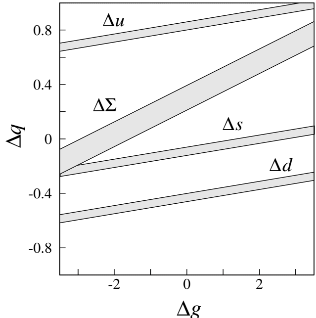
FIG. 22. Quark spin contributions to the proton spin as a function of the gluon contribution at Q^2 = 5 \text{ GeV}^2 in the Adler–Bardeen scheme.
