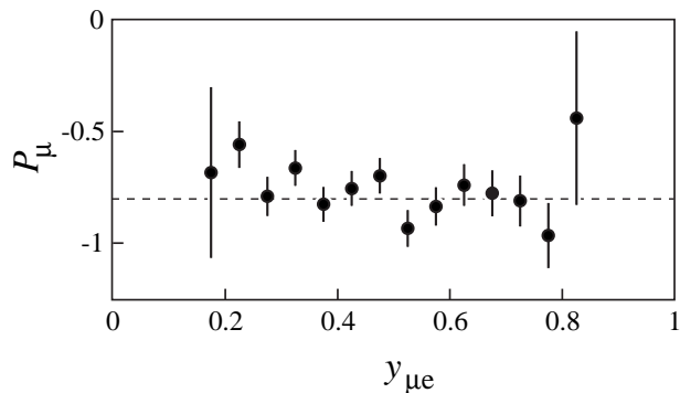
FIG. 7. Beam polarization vs. the ratio of electron and muon energies from polarized \mu - e scattering. The dashed line represents the average value.
