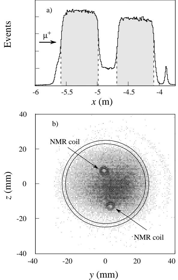
FIG. 10. Vertex distributions of scattered muons after kinematic cuts: (a) along the beam direction and (b) in the plane perpendicular to the target axis, at the location of one of the NMR coils. In (a), the dashed lines indicate the fiducial cuts on the target volume which coincide with the entry and exit windows of the target cells; most events outside the shaded region originate from interactions with the {}^3\text{He} - {}^4\text{He} cooling liquid. The small peak at x \approx -3.9\text{m} arises from scattering in the exit window of the target cryostat. In (b), the outer circle indicates the wall of the target cells, and the inner circle shows the radial cut applied. Scattering from the tubular NMR coils is clearly visible.
