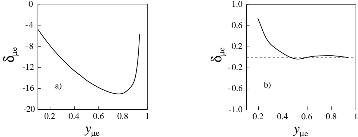
FIG. 6. The QED radiative corrections to the asymmetry A_{\mu e} (a) without experimental cuts. (b) The asymmetry if the following experimental cuts are included in the calculation: (i) recoil electron energy greater than 35 GeV, (ii) energy difference between initial and final states less than 40 GeV, (iii) angular cuts on both outgoing muon and electron. The corrections \delta_{\mu e} are given in percent.
