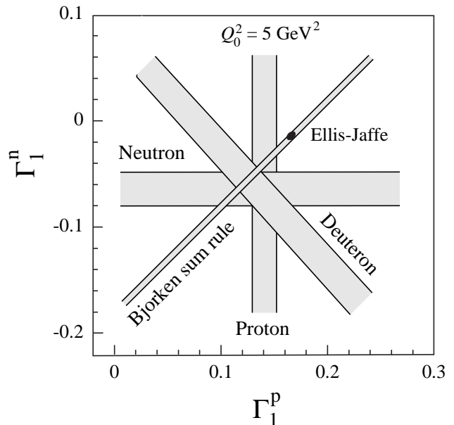
FIG. 21. Comparison of the combined experimental results for \Gamma_1^p , \Gamma_1^n and \Gamma_1^d with the predictions for the Bjorken and the Ellis–Jaffe sum rules. The Ellis–Jaffe prediction is shown by the black ellipse inside the Bjorken sum rule band.
