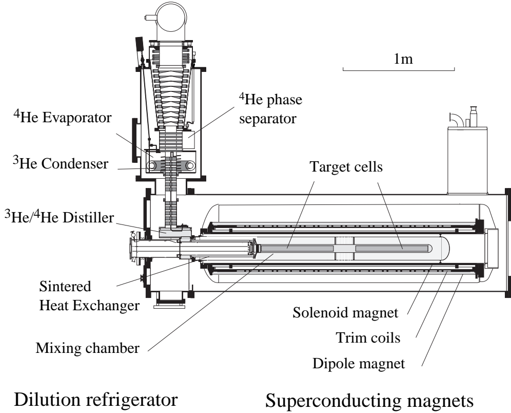
FIG. 8. Cross section of the SMC polarized target.
