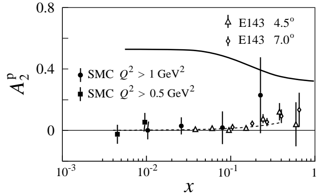
FIG. 15. Results for the asymmetry A_2^P(x) extrapolated to Q_0^2 = 5 \text{ GeV}^2 assuming \sqrt{Q^2}A_2^P scales [10]. The solid and dashed curves show the limit |A_2| < \sqrt{R} and the prediction corresponding to \bar{g}_2 = 0 , respectively. Also shown are data from the E143 experiment [41] extrapolated to the same Q_0^2 assuming that \sqrt{Q^2}A_2 scales. The errors are statistical only.
