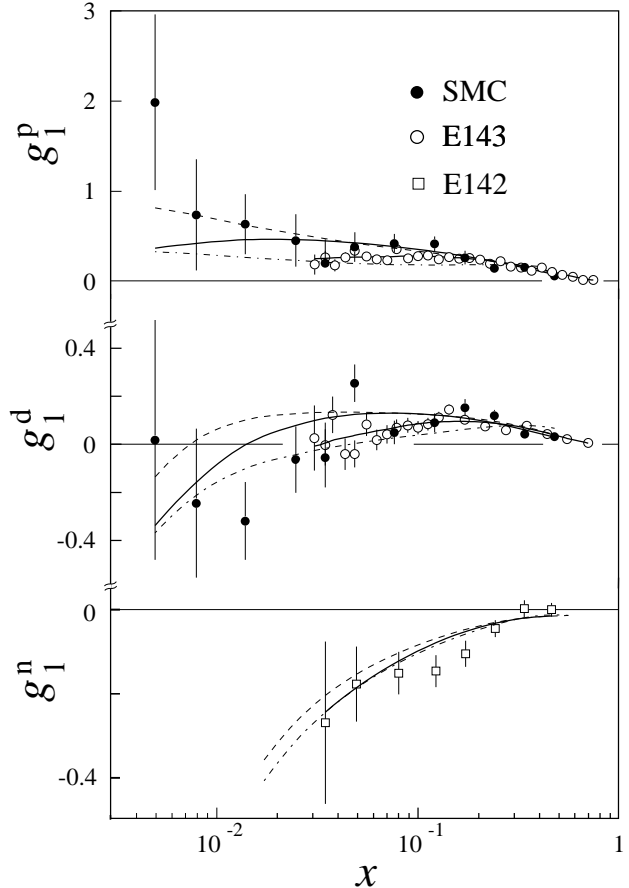
FIG. 17. The structure functions g_1^p , g_1^d , and g_1^n at the measured Q^2 for the SMC [13], E143 [6, 7] and E142 [107] data. The solid curves correspond to our NLO fits at the Q^2 of the data points, the dashed curve at Q_0^2 = 10 \text{ GeV}^2 , and the dot-dashed curve at Q_0^2 = 1 \text{ GeV}^2 .
