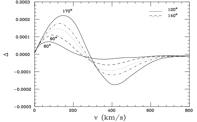
FIG. 3. Difference between velocity distributions of WIMP's of mass M_X = 50 \text{ GeV} for several angles \theta and the original Maxwell-Boltzmann distribution, \Delta = P_{MC}(v, \theta) dv - P_{MB}(v) dv . Here an interaction strength g = 10 was assumed.
