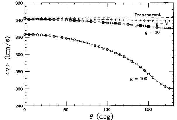
FIG. 4. Average velocity of WIMP's of mass M_\chi = 50 \text{ GeV} vs \theta . Three cases g = 3 , g = 10 , and g = 100 are compared to the average velocity of WIMP's going through a "transparent" Earth.
