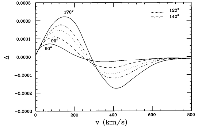
FIG. 3. Difference between velocity distributions of WIMP's of mass M_\chi = 50 \text{ GeV} for several angles \theta and the original Maxwell-Boltzmann distribution, \Delta = P_{\text{MC}}(v, \theta)dv - P_{\text{MB}}(v)dv . Here an interaction strength g = 10 was assumed.
