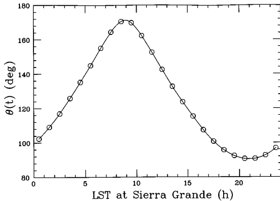
FIG. 2. Average variation of \theta(t) vs LST at Sierra Grande throughout the year of 1994. The coordinates of Sierra Grande are 41^\circ 40 \text{ min S} , 65^\circ 23 \text{ min W} .
