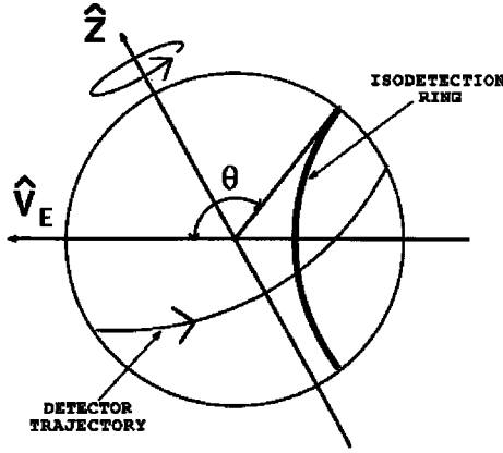
FIG. 1. Relevant directions in the scattering of WIMP's by the Earth as it travels around the galactic center with velocity \vec{V}_E . The angle \theta defines isodetection rings and a zenith angle.
