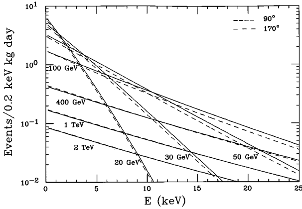
FIG. 5. Energy spectra for several masses at two different angles, \theta=90^\circ (day) and \theta=170^\circ (night). An interaction strength g=10 was assumed.
