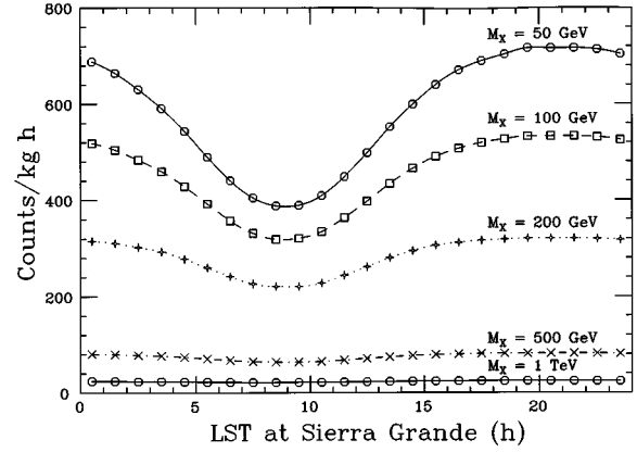
FIG. 6. Expected rate of events between E_{\min} and 50 keV for WIMP’s of different masses as a function of local sidereal time (LST) at Sierra Grande. An interaction strength of g=100 was assumed to make the diurnal modulation effect noticeable.
