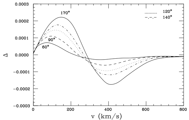
FIG. 3. Difference between velocity distributions of WIMP's of mass M_X = 50 \text{ GeV} for several angles \theta and the original Maxwell-Boltzmann distribution, \Delta = P_{MC}(v, \theta)dv - P_{MB}(v)dv . Here an interaction strength g = 10 was assumed.
