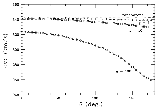
FIG. 4. Average velocity of WIMP's of mass M_X = 50 \text{ GeV} vs. \theta . Three cases g = 3 , g = 10 , and g = 100 are compared to the average velocity of WIMP's going through a "transparent" Earth.
