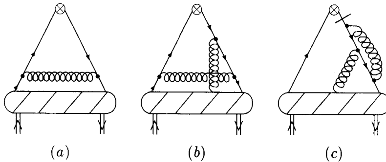
Figure 5: One-loop radiative corrections for two-particle correlators in the Abelian gauge theory. The fermion propagator crossed with a bar on diagram (c) shows the contraction of the corresponding line into the point.
