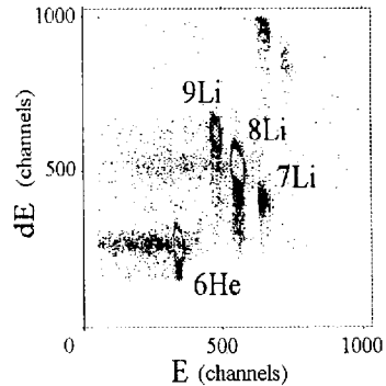
Figure 5. \Delta E -E beam matrix for the beam tuned to optimal yield of ^6\text{He} ions
