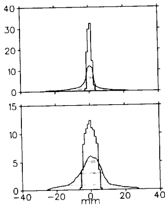
Figure 3. The same profiles as in Fig. 2 but in the achromatic focal plane F_3 . The measured FWHM widths are 5 and 12 mm, respectively. The calculated profiles are simulated for beam momentum spread of 1.3%. The object slit is as in Fig. 2.
