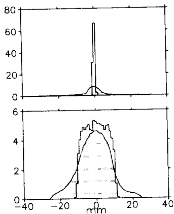
Figure 2. The horizontal (top) and vertical (bottom) ^{14}\text{N} beam profiles (histograms - calculated, smooth curves - measured) in the intermediate focal plane F_2 . The measured FWHM are 7 and 20 mm, respectively. The calculated profiles are simulated for the monochromatic beam. The main object slit is equal to 3 \times 10 \text{ mm}^2 .
