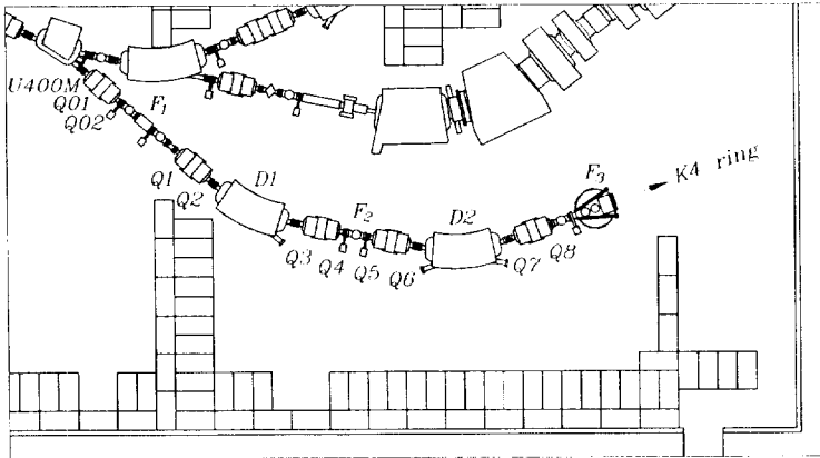
Figure 1. The ACCULINNA beam line.
