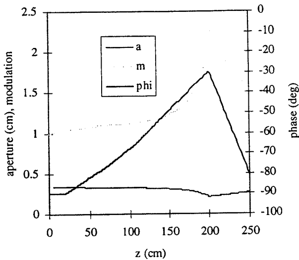
Fig. 1. Variation of RFQ aperture, modulation and phase vs. length. Phase and modulation are tapered down in the last section in order to limit the output energy to 100 keV/u for the first phase of the experiment.
