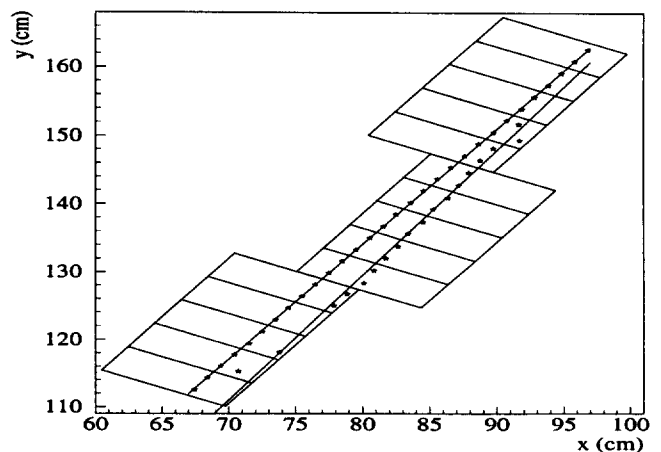
Fig. 7 Laser induced tracks in the TPC outer sector. The area instrumented with electronics is also shown.
