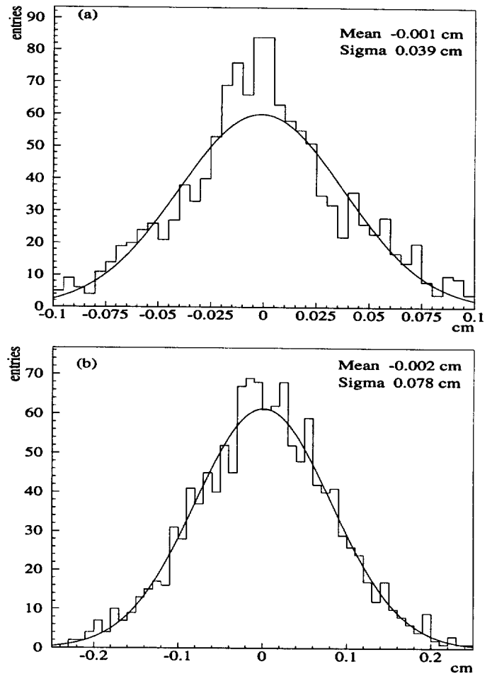
Fig. 6 Particle hit residuals in the (a) azimuthal and (b) drift direction.
