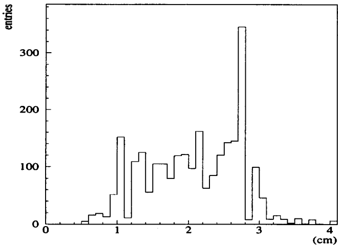
Fig. 8 Two-track hit separation from laser induced ionization events. While tracks are created with up to 3 cm separation, they are seen to merge below a separation of \sim 1 cm.
