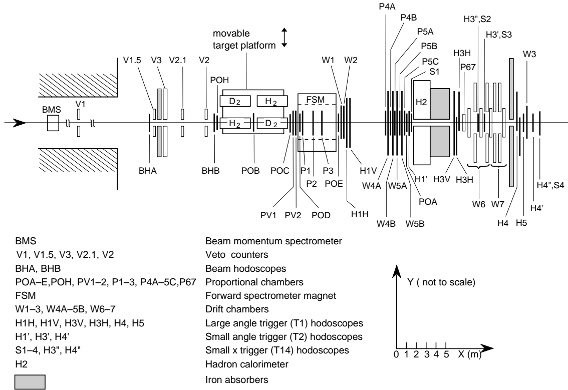
Figure 1: The NMC spectrometer for the 1989 data taking. The beam calibration spectrometer is located downstream and not shown.
