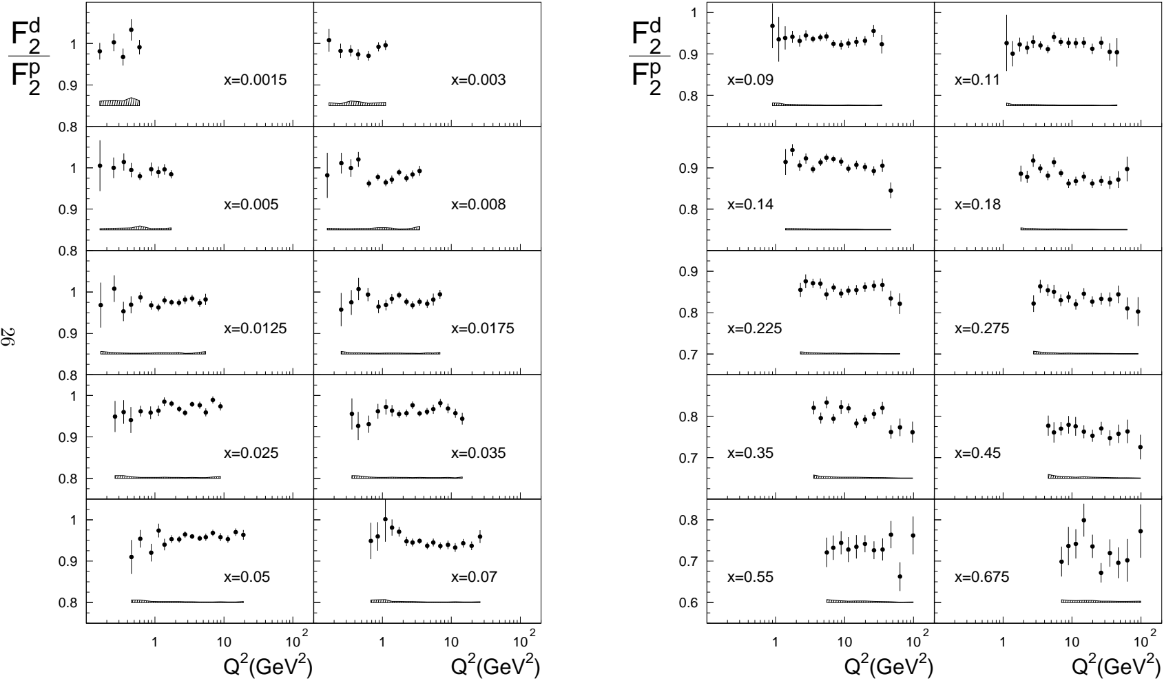
Figure 5: The structure function ratio F_2^d/F_2^p as a function of Q^2 for each x bin. The error bars represent the statistical uncertainties and the size of the systematic errors is indicated by the bands.
