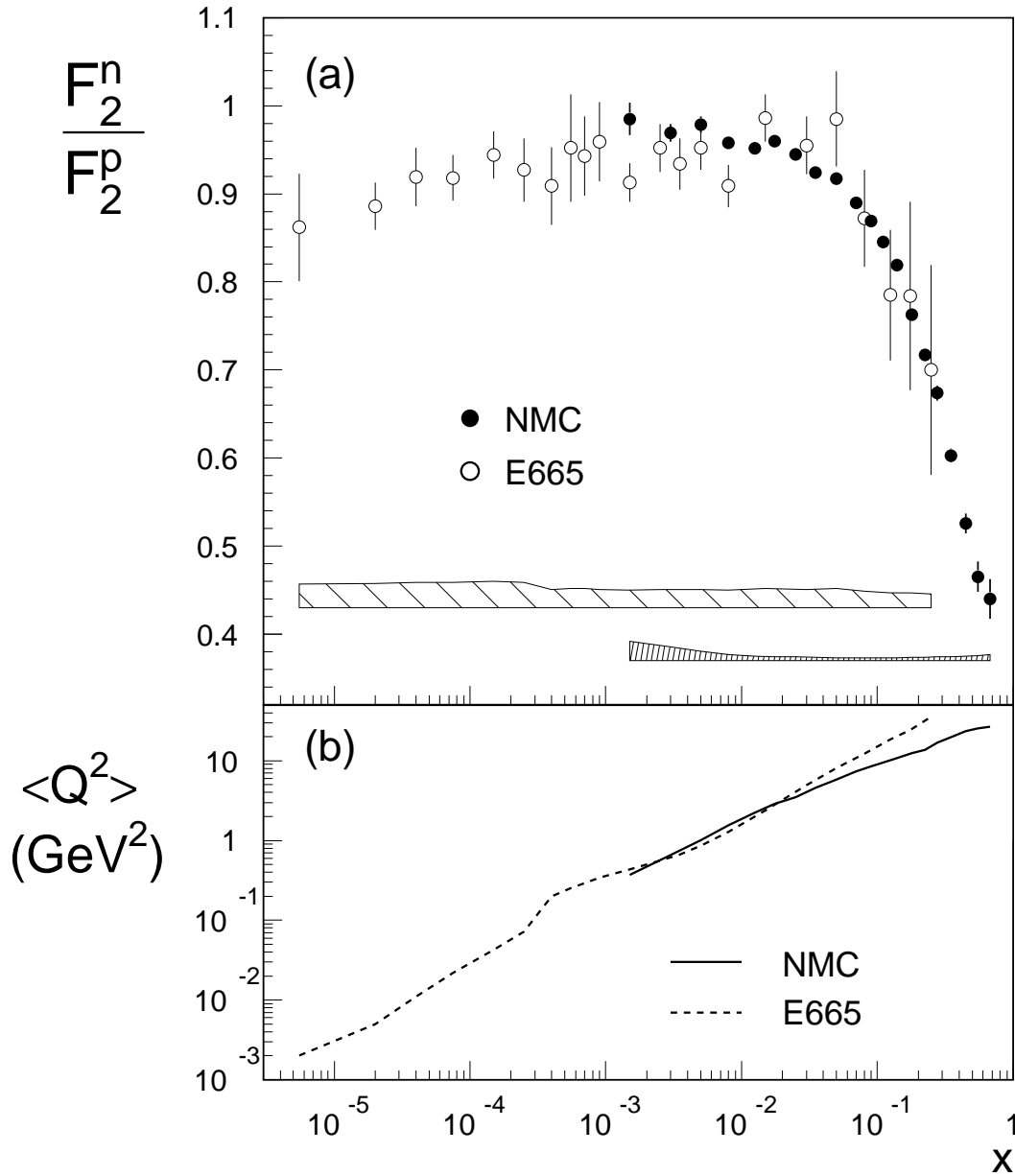
Figure 9: (a) Comparison of the x dependence of the present data for F_2^n/F_2^p with the results from the E665 collaboration [39]. The error bars represent the statistical errors and the bands at the bottom indicate the systematic uncertainties. (b) The average Q^2 of the E665 and the present data versus x .
