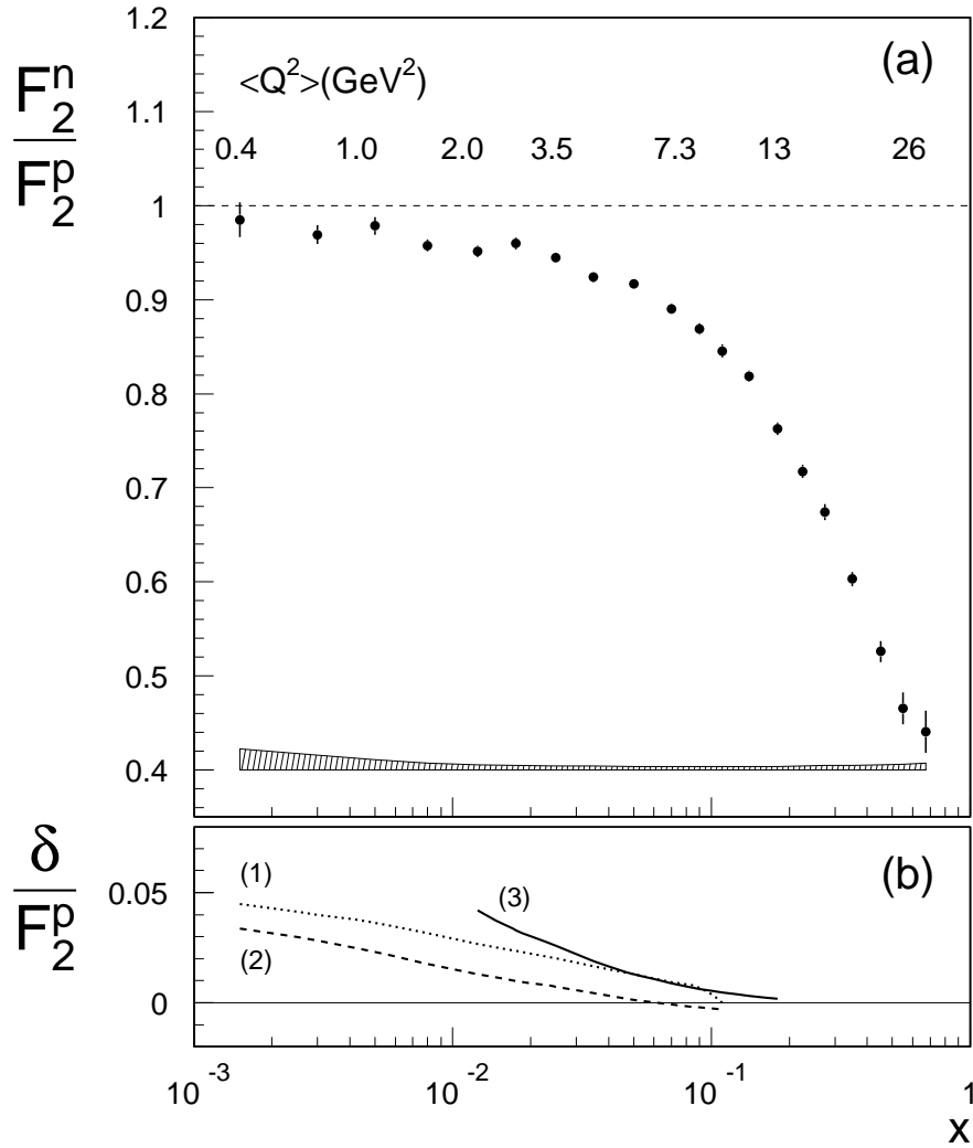
Figure 8: (a) The structure function ratio F_2^n/F_2^p as a function of x . The error bars represent the statistical errors and the band at the bottom indicates the systematic uncertainty. The numbers given across the top of the figure are the average Q^2 values. (b) Model predictions for \delta/F_2^p , the corrections to F_2^n/F_2^p due to shadowing in the deuteron, from ref. [33] line(1), ref. [34] line (2) and ref. [35] line (3).
