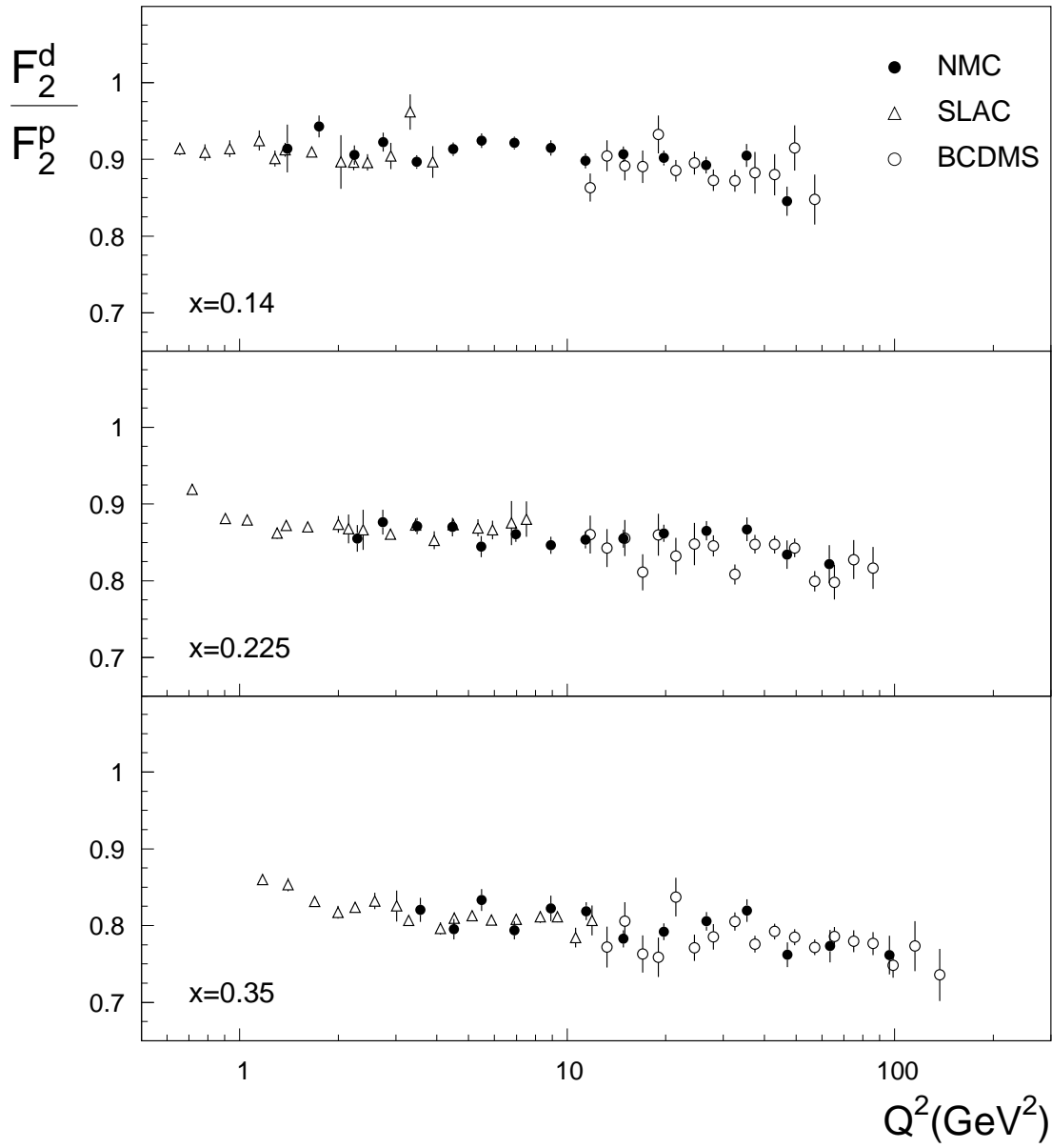
Figure 6: Comparison of the present results with the ones from SLAC [29] and BCDMS [30] for selected x bins. The SLAC data were rebinned in x and Q^2 . The error bars represent the statistical uncertainties.
