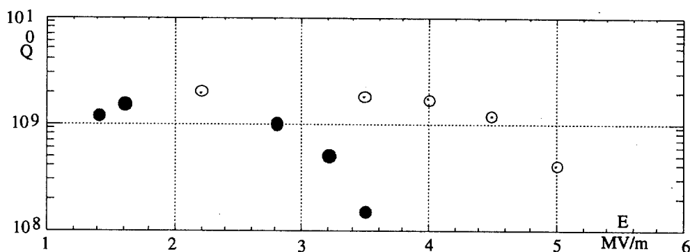
Figure 10 – Q_0 vs. accelerating field E @ 4.2 K.
