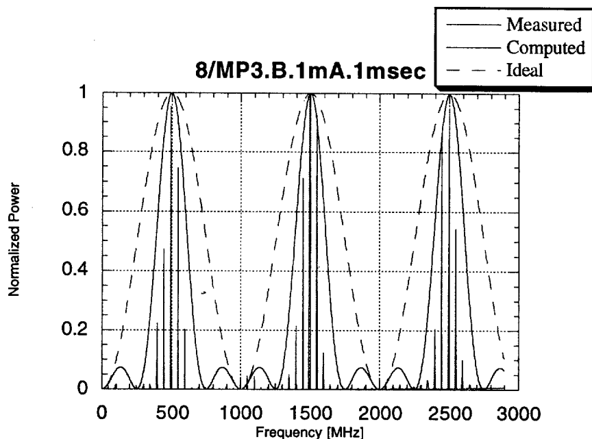
Figure 7 – Measured spectrum lines, computed and ideal envelopes.
