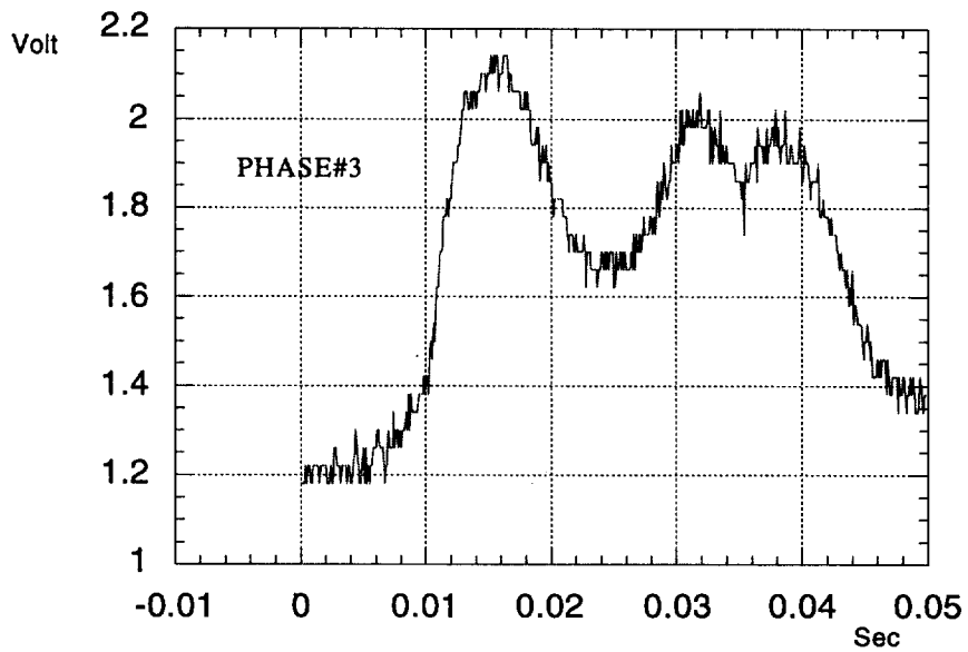
Figure 15 –Typical phase error signal during pulse (1Volt=5 degrees).
