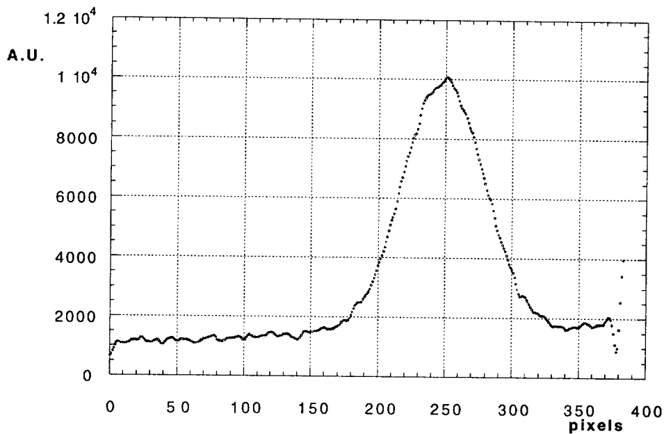
Figure 20 – Horizontal beam profile from previous image.
