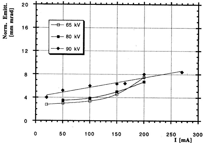
Figure 4 – Gun emittance vs. current.
