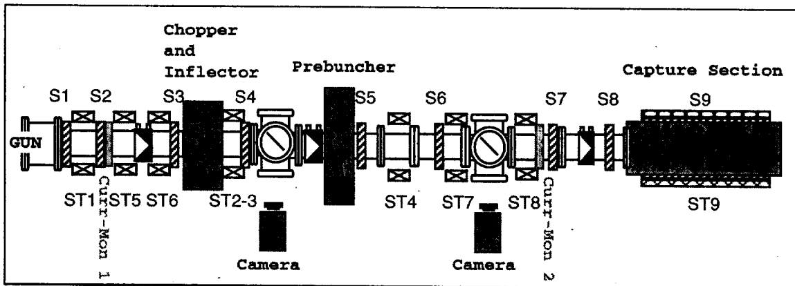
Figure 3 - Injector line.
