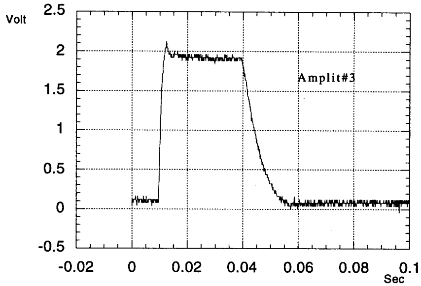
Figure 14 – Typical voltage pulse(1 V=1.5 MV).
