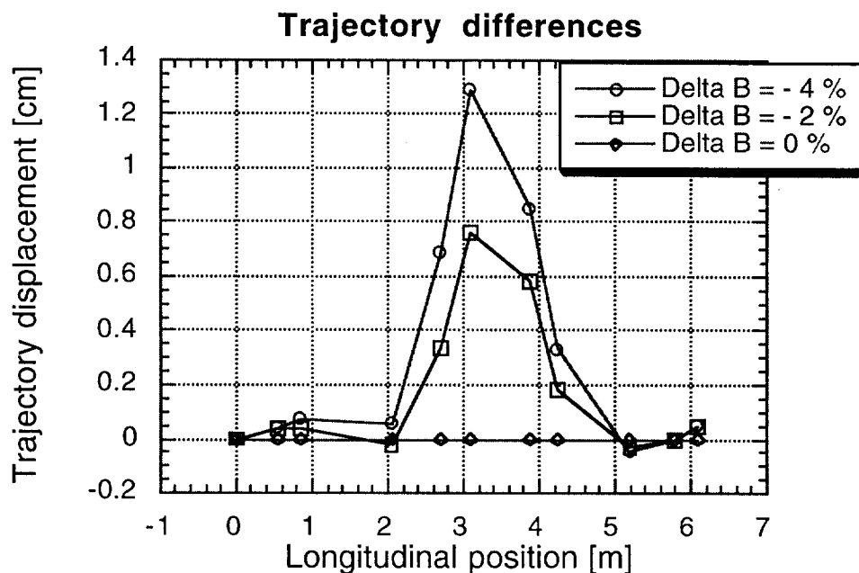
Figure 21 – BPM measurement of the relative beam displacement in the arc varying the bending field of -2% (square points) and -4% (dot points).
