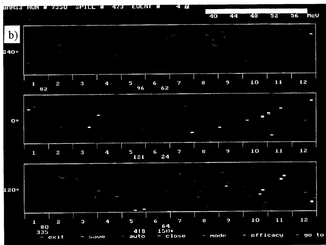
Fig.6. Background events from EAS(a) and a group of muons(b). Scale of energy deposited in the cells is shown at the top of figs.
