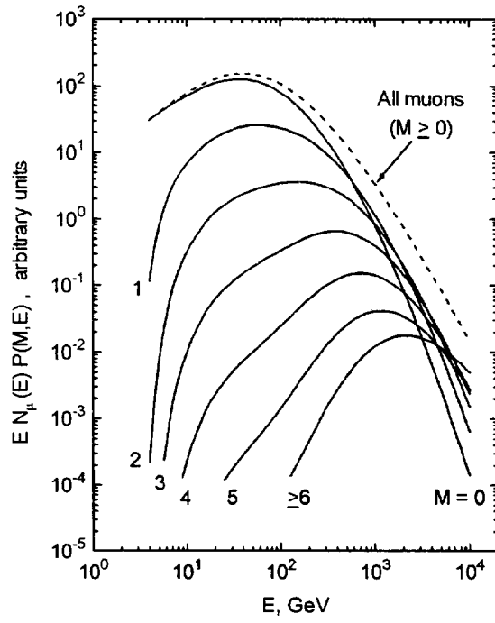
Fig. 10. Calculated spectra of cosmic ray muons corresponding to fixed number of interactions M with energy transfers \varepsilon > 1 GeV. P(E, M) is the probability to produce M interactions for muon with energy E .
