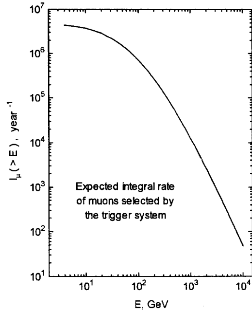
Fig. 12. Expected muon flux per year through one BARS.
