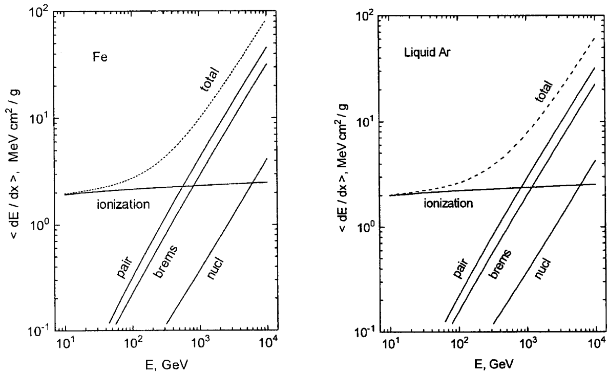
Fig. 1. The average energy loss of muons in iron and liquid argon as a function of energy.
