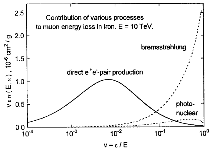
Fig. 2. Energy loss distributions of 10 TeV muon for e^+e^- production, bremsstrahlung, and photonuclear interaction.
