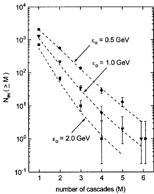
Fig. 11. Distribution of EM shower multiplicities for different values of the energy threshold \varepsilon_0 .
