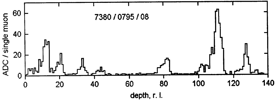
Fig. 8. Energy distribution along the BARS for the event shown in fig. 7b.
