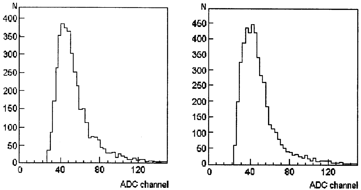
Fig. 5. Typical pulse height distributions for relativistic muons.
