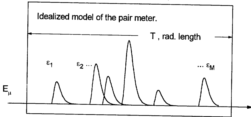
Fig. 3. Longitudinal energy distribution in the ideal pair meter.
