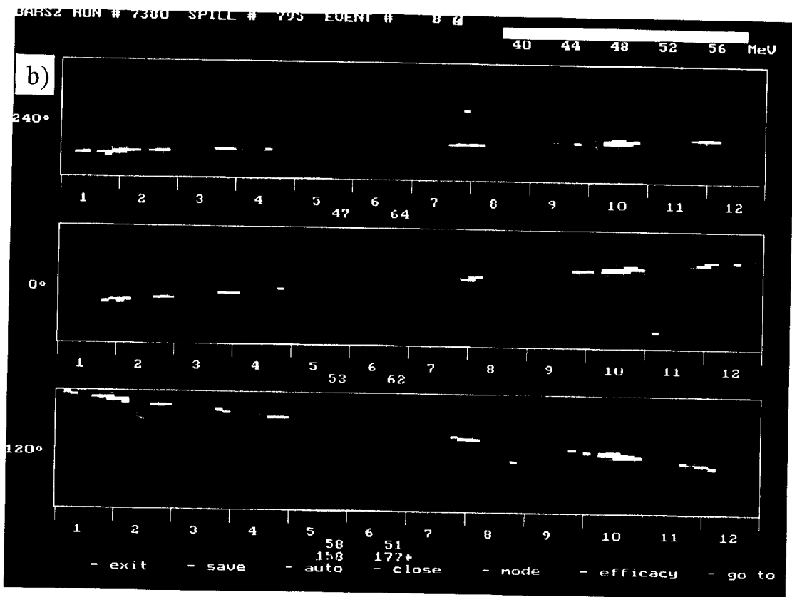
Fig. 7. Muon tracks. Scale of energy deposited in the cells is shown at the top of figs.
