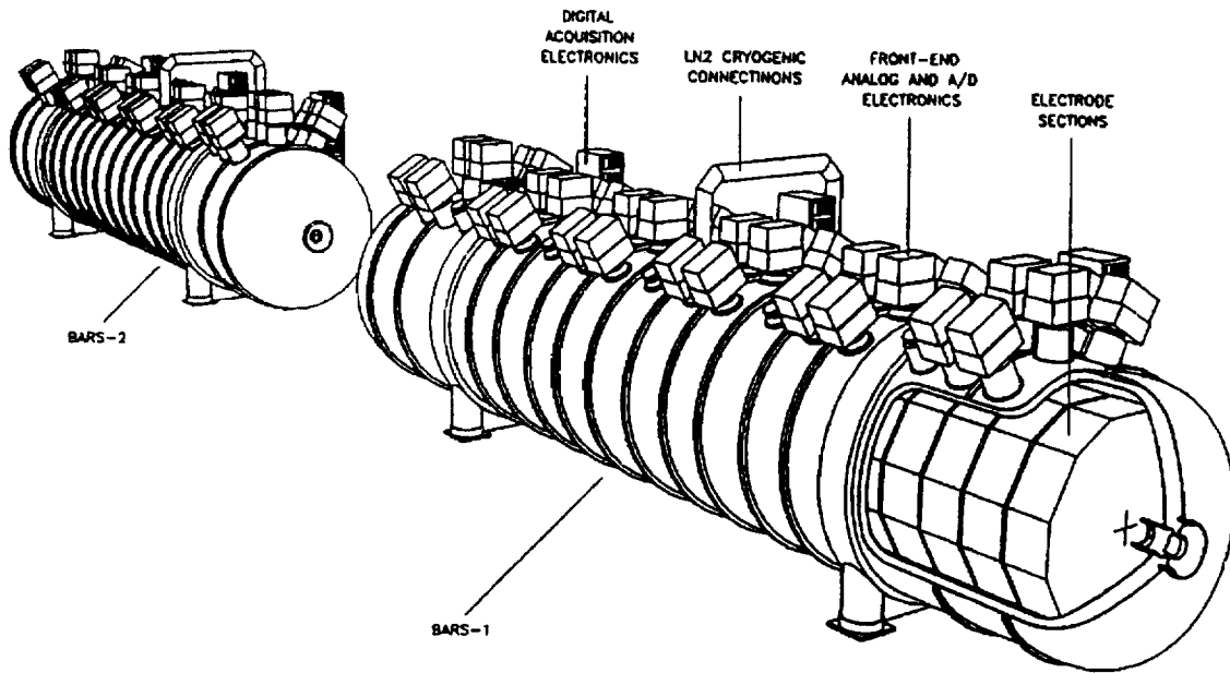
Fig. 4. BARS calorimeters.
