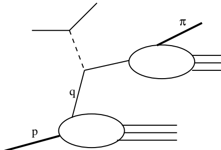
Figure 3: Parton model for semi-inclusive DIS.
