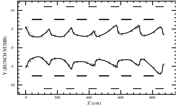
Fig. 5. Envelope in the Y plane (mm).
