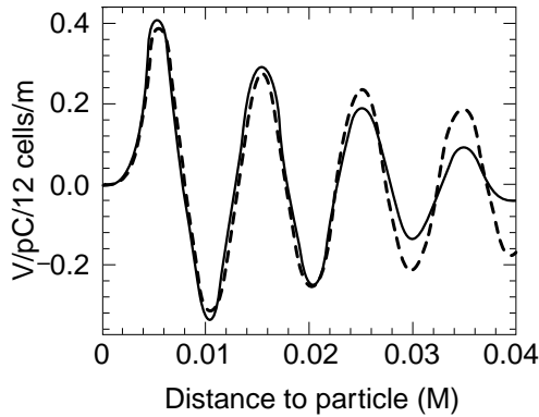
Fig. 3. Wake from MAFIA (dashed) and convolution (cont.).
