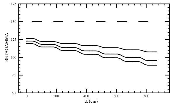
Fig. 4. Minimum, average, maximum energies in bunch 12.
