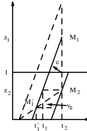
Fig. 1. Forward wake
