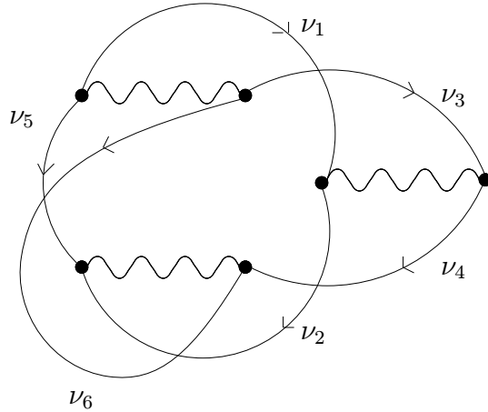
Figure 2: Vanishing cycles for N_f = 4
