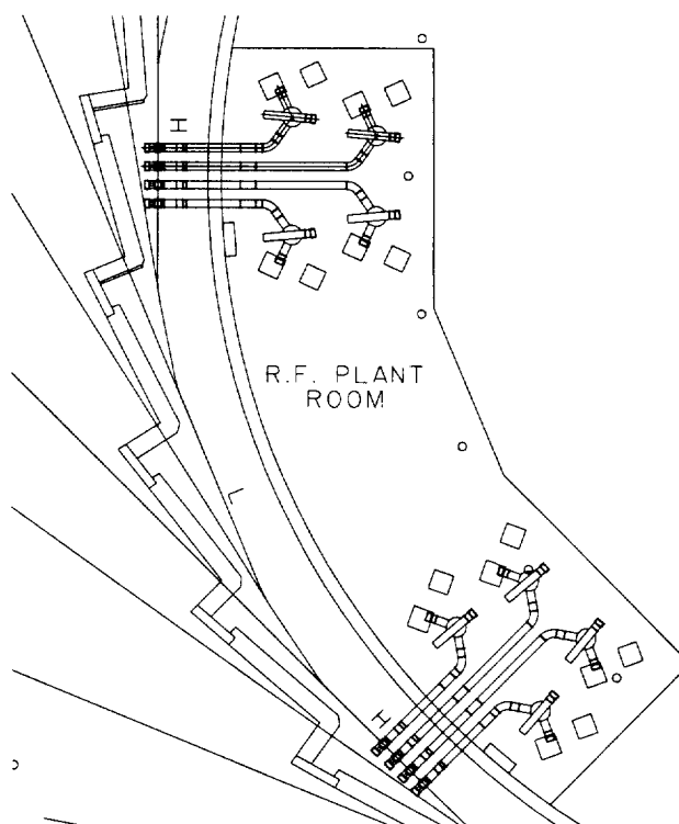
Figure 1. RF Layout.
