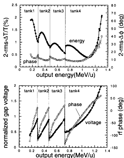
Figure 1: Upper part is the minimum energy spread and the corresponding phase spread at the exit of the each tank as a function of the output energy. Lower one is the gap voltage and the rf phase to give the minimum energy spread (the rf phase 0 means that particles are injected in a synchronous phase( -25^\circ )).
