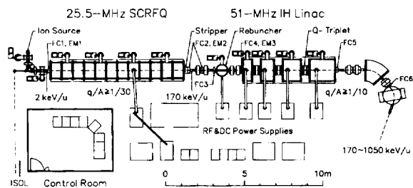
Figure 4: Layout of the linac complex.
