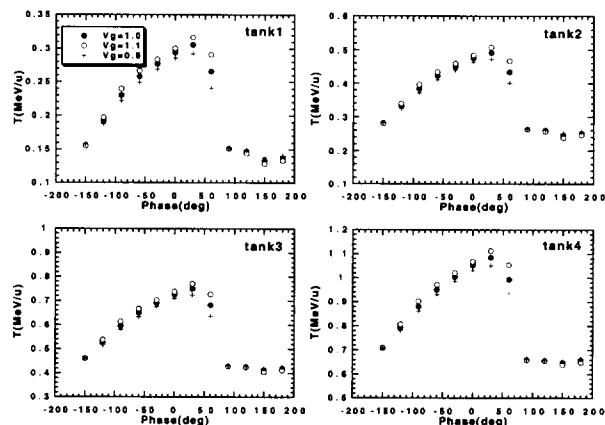
Figure 6: Dependence of the output energy on the rf phase (by a simulation).
