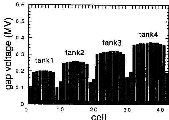
Figure 2: Gap voltage distributions measured by a bead-pull method. The gap voltage is given by the nominal maximum one.
