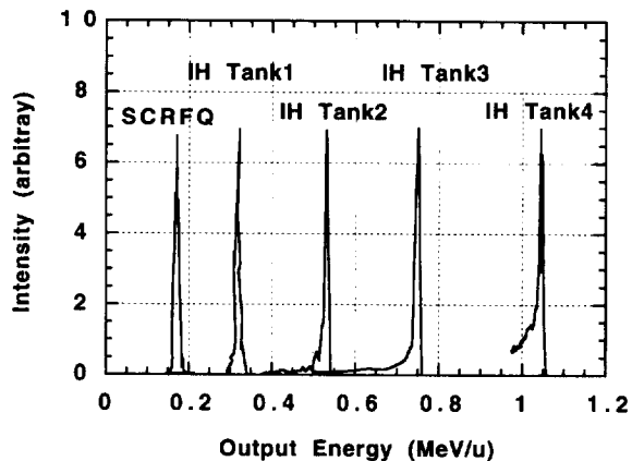
Figure 5: Momentum analyzed beam for five acceleration modes.
