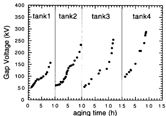
Figure 3: Aging history of the IH linac.
