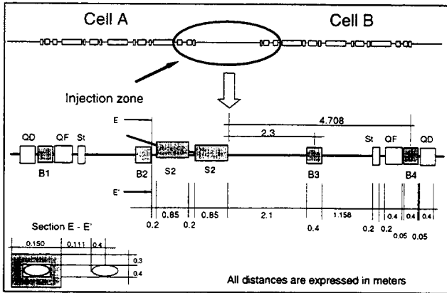
Figure 1. Injection scheme for the LSB storage ring.
