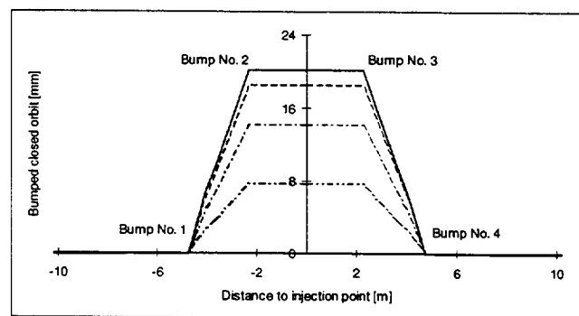
Figure 3. Bump amplitude during the 4 first turns. Positive Y axis points towards the center of the ring.
