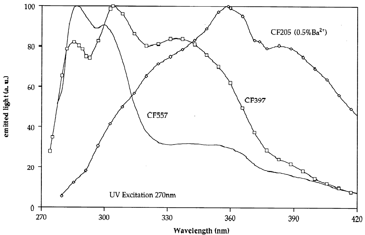
Fig. 5: Photoluminescence spectra for different CeF_3 crystals
