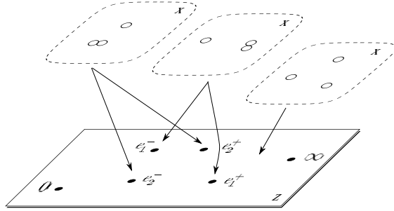
Fig.1. The Seiberg-Witten curve can be understood as fibration of a weight diagram over \mathbb{P}^1 . Pairs of singular points in the base are associated with vanishing 0-cycles in the fiber, i.e., to root vectors a_i - a_j . In string theory, the local fibers are replaced by appropriate ALE spaces with corresponding vanishing two-cycles. As will be explained in the next section, this picture has a natural interpretation in terms of D-branes.
