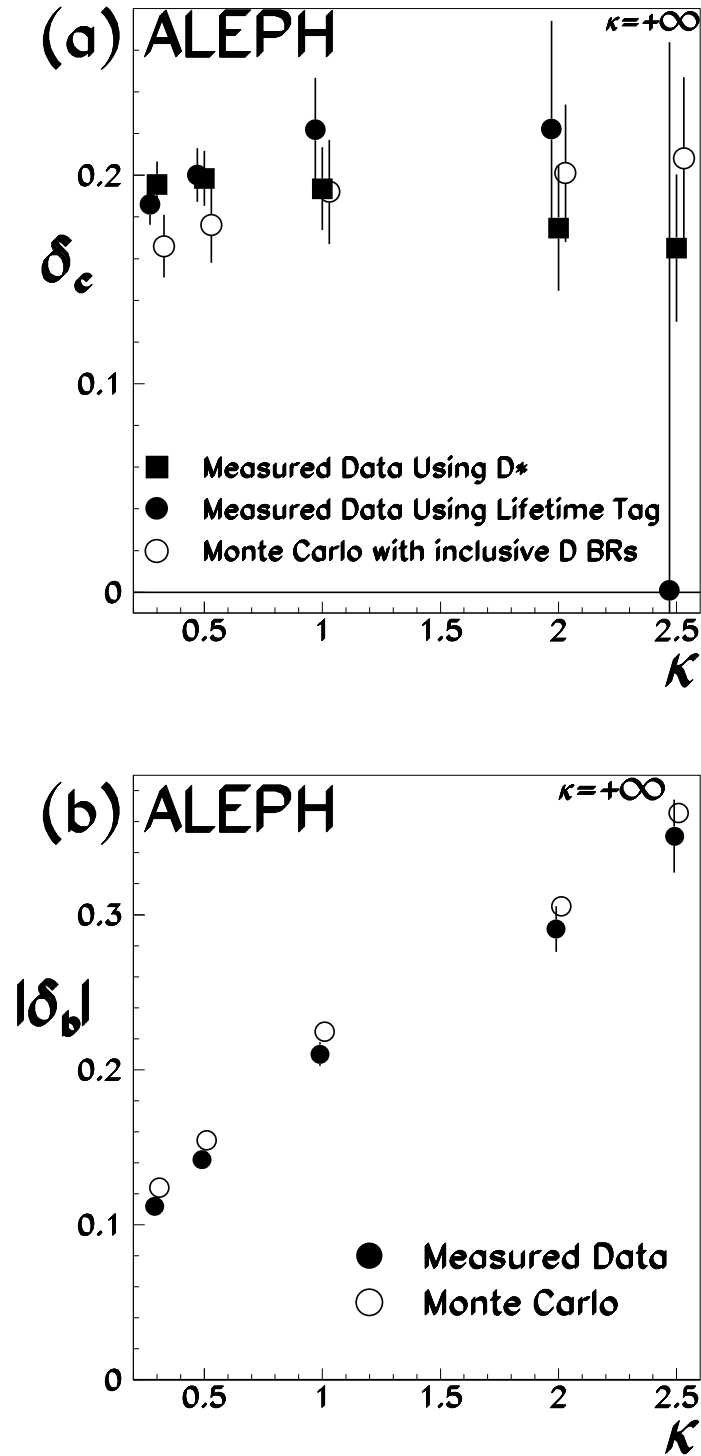
Figure 3: (a) Comparisons of the lifetime tag and D^{*\pm} measurements of \delta_c and with that expected from Monte Carlo simulation. (b) Comparison of the lifetime tag measurement of \delta_b with that expected from Monte Carlo simulation.
