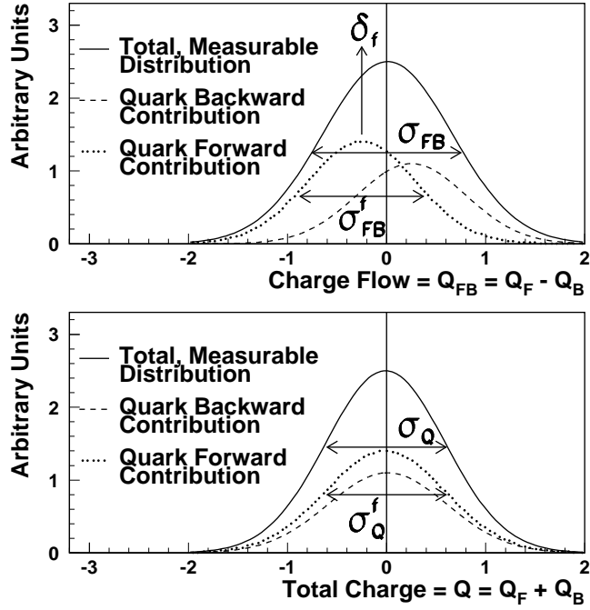
Figure 1: Illustration of the Q_{\text{FB}} and Q charge distributions for a quark of flavour f . The widths of the Q_{\text{FB}} and Q distributions in the case the quark f goes forward, \sigma_{\text{FB}}^f and \sigma_Q^f , are approximately equal if the correlations between hemispheres are small.
