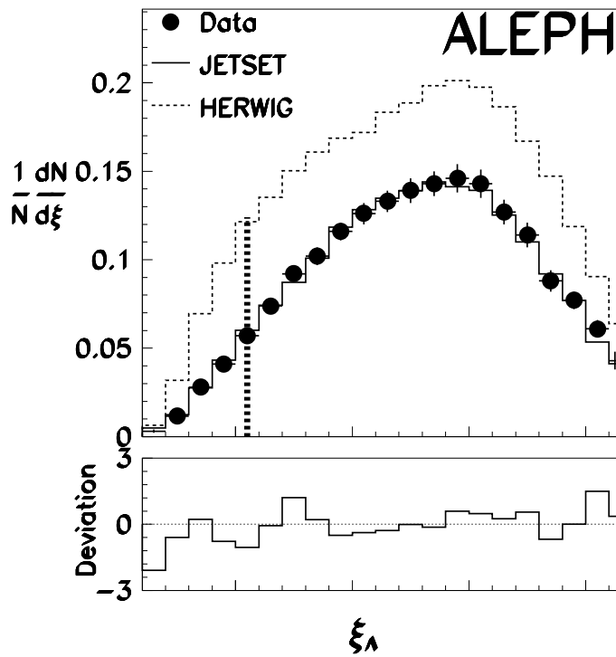
Figure 10: As for the previous figure but for the \Lambda spectrum. A deweighting factor of 500 is used for HERWIG in this case.
