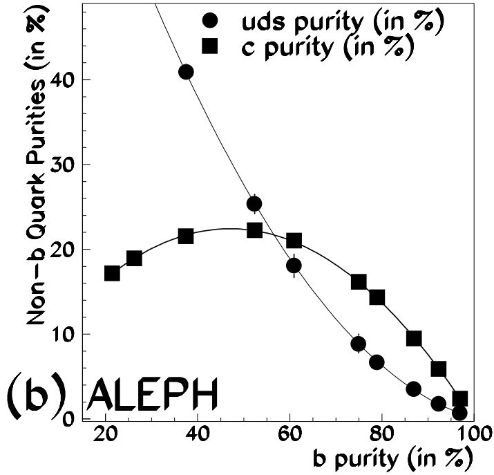
Figure 2: (a) Measured values of \bar{\delta} are plotted as a function of b purity. Results are shown for a variety of \kappa values. (b) Light ( u, d, s ) and c quark purities as a function of the b purity \mathcal{P}_b . The curves are parameterisations.
