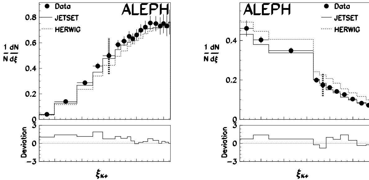
Figure 8: As for the previous figure but for the charged kaon spectrum. A deweighting factor of 24 is used for HERWIG in this case.
