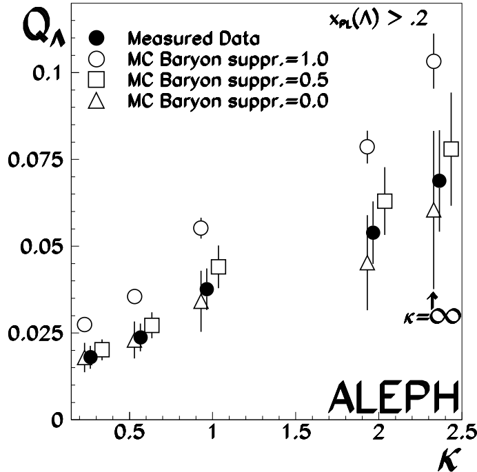
Figure 11: Comparison of the charge opposite a \Lambda to the JETSET prediction plotted as a function of \kappa and for x_\Lambda = p_\Lambda/E_{\text{beam}} > 0.2 . The JETSET Monte Carlo is compared to the data for various settings of the fast baryon suppression parameter.
