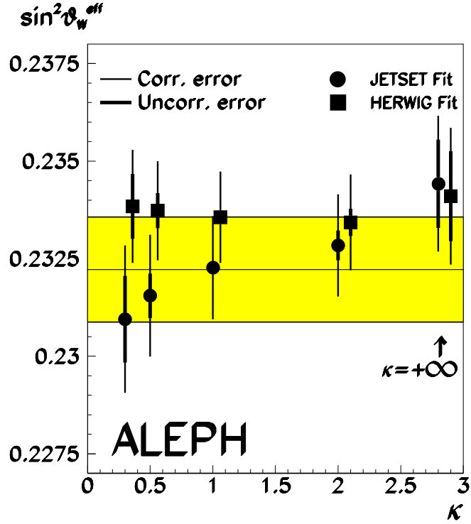
Figure 12: The value of \sin^2 \theta_w^{\text{eff}} plotted as a function of \kappa using separations both from the JETSET and HERWIG Monte Carlos and \langle Q_{\text{FB}} \rangle for the Z peak energy. The errors (thick lines) shown are relative to the value obtained at \kappa = 1.0 . The errors for each point are indicated by the extensions (thin lines) of the errors. The shaded region represents the final result with its total error. The systematic errors given in Tables 16 and 17 are not included in the points in the figure. Since they are not fully correlated as a function of \kappa , they could be responsible for some of the variations of \sin^2 \theta_w^{\text{eff}} with \kappa .
