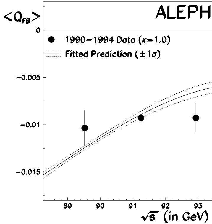
Figure 13: \langle Q_{FB} \rangle plotted as a function of centre-of-mass energy for the data (points) and a prediction using the fitted values of the JETSET light quark charge separations, the measured values of the heavy quark charge separations and the fitted value of \sin^2 \theta_w^{\text{eff}} . The family of curves reflects the errors on the quark charge separations. The results are shown for \kappa = 1.0 .
