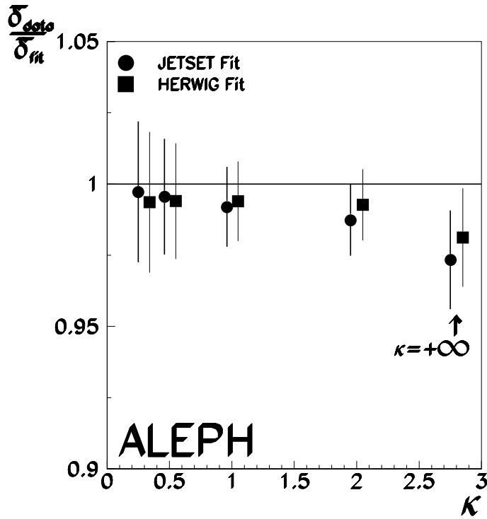
Figure 6: The ratio of \bar{\delta} in the data to that fitted from the Monte Carlo, plotted as a function of \kappa for JETSET and HERWIG fits. Error bars represent the statistical and systematic uncertainties in data and the statistical error on the Monte Carlo.
