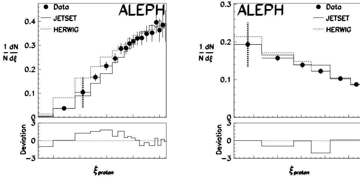
Figure 9: As for the previous figure but for the proton spectrum. A deweighting factor of 30 is used for HERWIG in this case.
