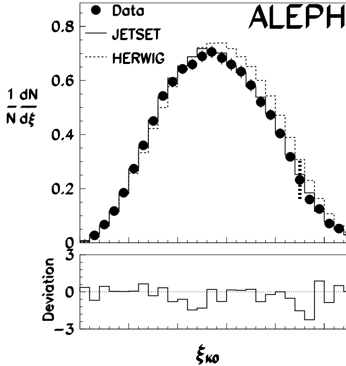
Figure 7: Neutral kaon spectrum compared to the JETSET (solid) and HERWIG (dashed) Monte Carlos. The spectrum is described in terms of the momentum fraction of the beam energy that the neutral kaon carries by \xi = -\log(p/E_{\text{beam}}) . The dashed error bar gives one example of the deweighting factor of 30 in the \chi^2 used for the HERWIG fit. No deweighting is used for JETSET. The number of standard deviations of the JETSET prediction from the data is shown by the solid line in the lower portion of the figure and includes statistical and systematic errors added in quadrature.
